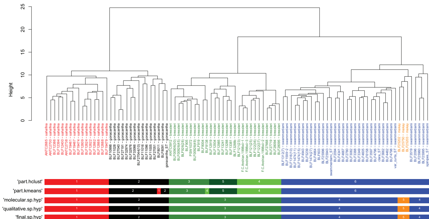
Dendrogram of agnes(x = mpredlda, method = "average")
