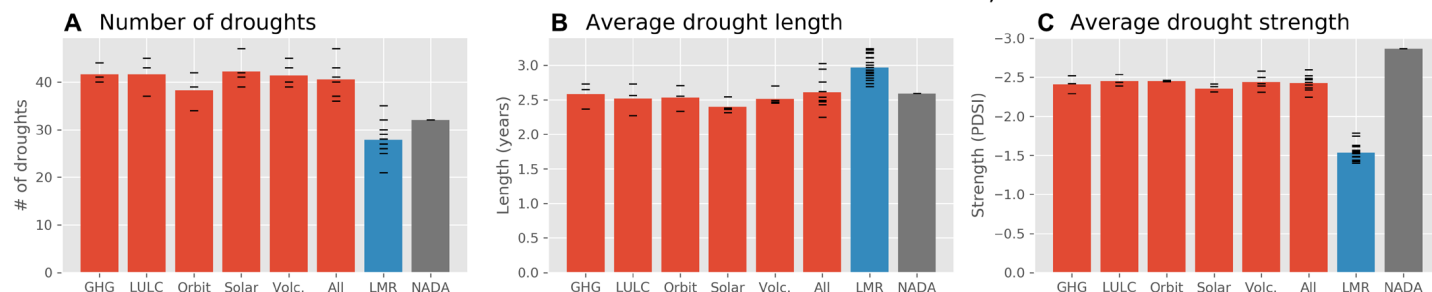
Fig. 6. PDSI statistics in different experiments. Statistics of annual-mean PDSI in the southwest United States in different CESM-LME simulations, LMR, and NADA. Bar plots show the (A) number of droughts, (B) average drought length, (C) and average drought strength for years 850 to 1849 C.E. Colored bars show the ensemble-mean values for each experiment type, with black dash marks showing the values for each ensemble member. The LMR and NADA results are shown in different colors to call attention to the different methodologies used. GHG, greenhouse gases; LULC, land use/land cover; Orbit, Earth's orbit; Solar, solar irradiance; Volc, volcanic forcing.
