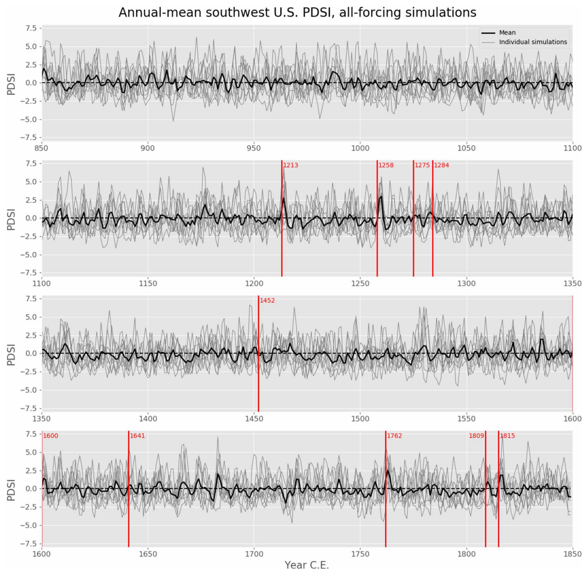
Fig. 5. Southwest U.S. PDSI in CESM-LME. Time series of PDSI averaged over the southwest United States (land within 32°N to 40°N, 125°W to 105°W) in the nine all-forcing simulations, as well as their mean. Years of the 10 largest volcanic forcings are marked; these vertical lines mark the first year of a large volcanic aerosol forcing, so the year listed may not exactly match the year of the actual eruption.
