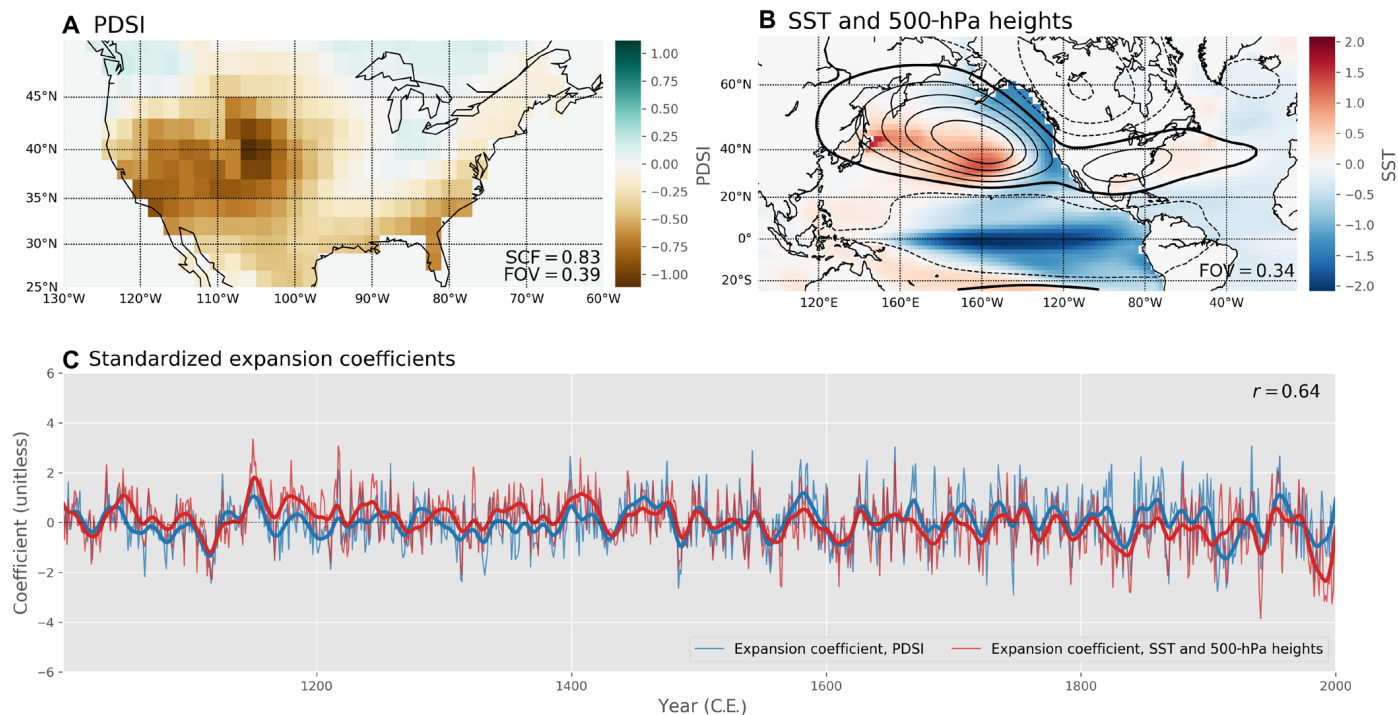
Fig. 3. MCA. MCA between PDSI and SST/500-hPa heights for mode 1. (A and B) Maps showing the spatial patterns of variability and (C) standardized expansion coefficients showing how the magnitudes of the spatial patterns change through time. In (B), positive height anomalies are indicated by solid contours and negative anomalies are indicated with dashed contours, with the thicker line indicating 0. SSTs and 500-hPa heights are standardized before conducting this analysis, so the values shown are not covariances. Calculations are performed on the data in the regions shown. The squared covariance fraction (SCF; measuring the amount of squared covariance for which each mode accounts) as well as the fraction of variance (FOV; measuring the relative amount of variability explained by this mode for the variable under consideration) are listed in the lower right of (A) and (B). The correlation ( r ) of the expansion coefficients is given in (C).
