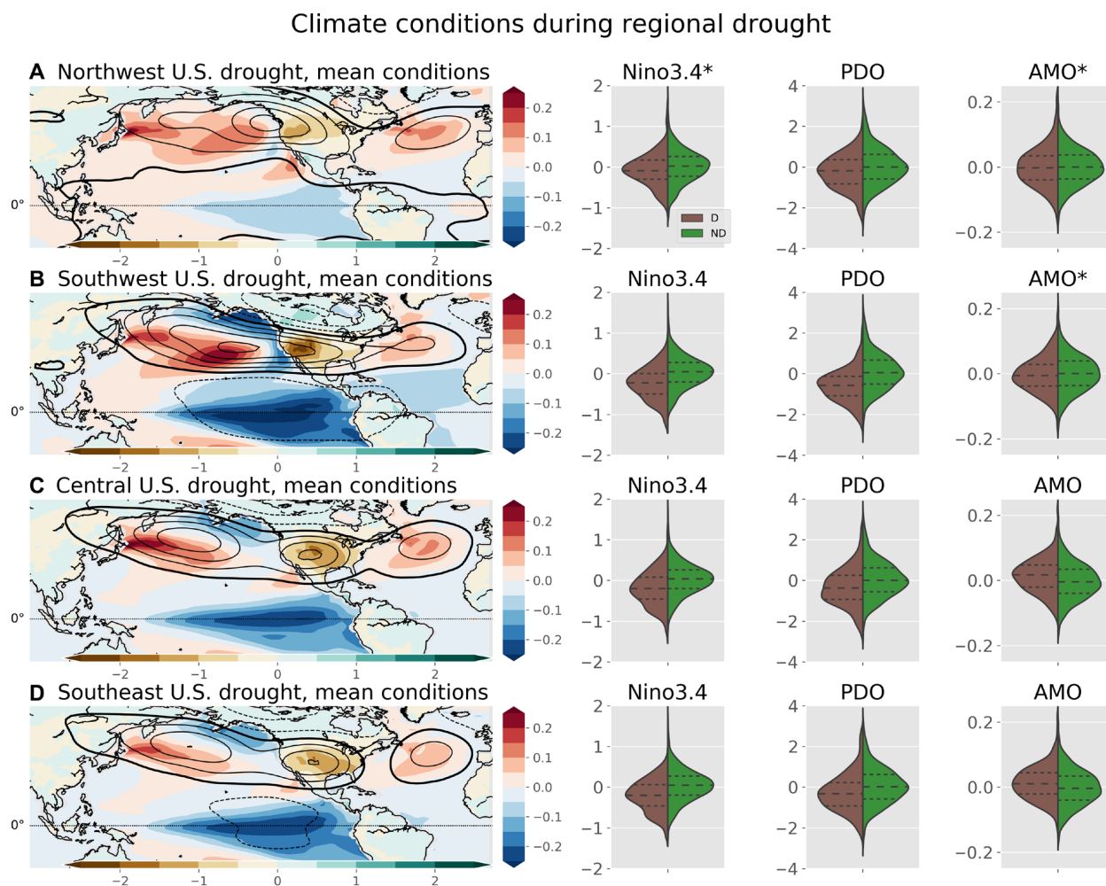
Fig. 4. Climate fields associated with regional drought. Maps show mean SST (°C), 500-hPa heights (hPa), and PDSI for drought years relative to all years in four U.S. regions: (A) northwest, (B) southwest, (C) central, and (D) southeast United States. The contour interval for 500-hPa heights is 2 hPa, with the thicker line indicating 0. Split violin plots show distributions of annual-mean values of Nino 3.4, PDO, and AMO for drought years (brown) versus nondrought years (green) in each region, with lines indicating the medians and interquartile range. Differences in means between drought years and nondrought years that are not significant according to a resampling test at the 95% level (Materials and Methods) are indicated with an asterisk next to the name of the climate index.
