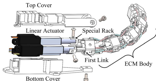
Fig. 5 Overall design of the new ECM
