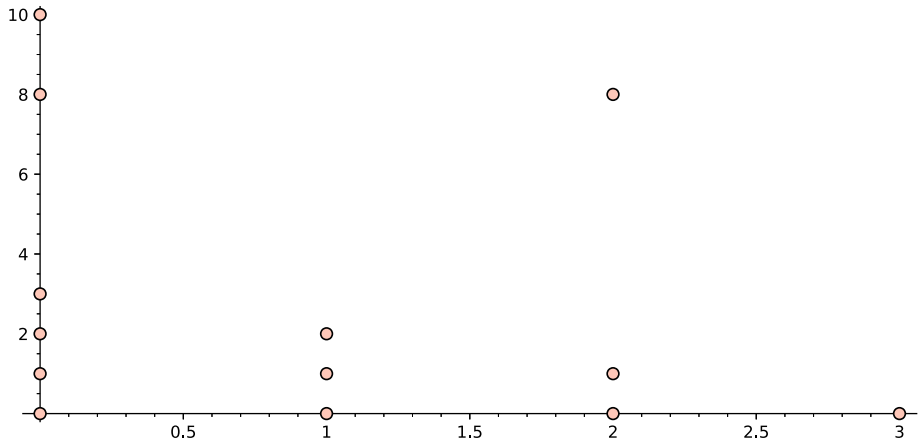
Fig. 1 Exponent pairs (a, b) with x^a y^b \in \mathcal{C} for q = 4 ( a is on horizontal axis)
