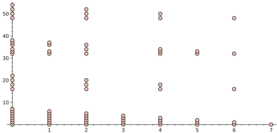
Fig. 2 Exponent pairs (a, b) with x^a y^b \in \mathcal{C} for q = 8 ( a is on horizontal axis)
