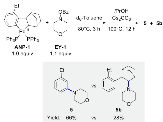
Fig. 1 Pd/NBE-catalyzed arene C–H amination with N -benzoyloxycarbonylamine.
