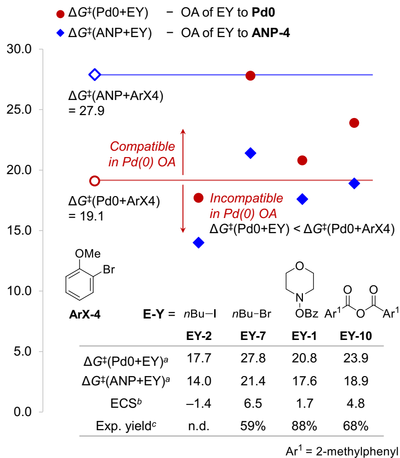
Fig. 6 Computationally predicted electrophile compatibility scores (ECS) of electrophiles with 2-bromoanisole ( ArX-4 ). a All energies are in kcal/mol with respect to Pd0 or ANP-4 . b Electrophile compatibility score between each electrophile and ArX-4 . c Experimental yields from ref. 14.
