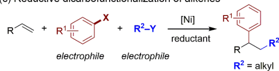
(c) Reductive dicarbofunctionalization of alkenes
