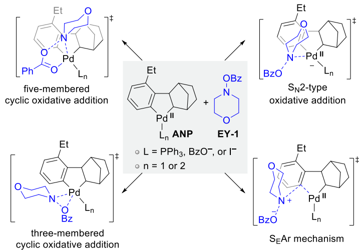
(b) Possible mechanisms for the reaction of ANP with electrophile EY-1
