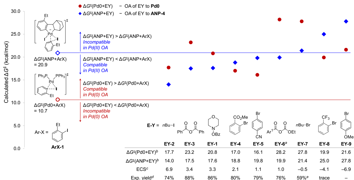
Fig. 5 Computational predictions of compatibility of electrophiles (EY) in the Pd/NBE-catalyzed reactions with ortho -ethyl iodobenzene ( ArX-1 ). a Ar 1 = 2,6-dimethylphenyl. b All energies are in kcal/mol with respect to Pd0 or ANP-4 . c Electrophile compatibility score between each electrophile and ArX-1 . d Experimental yields from refs. 26, 38, 34, 31, 39 were from reactions with 2-iodotoluene unless otherwise noted. e Experimental yield was from the reaction with 2-bromoanisole.
