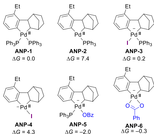
(a) Possible ANP species under the catalytic conditions a
