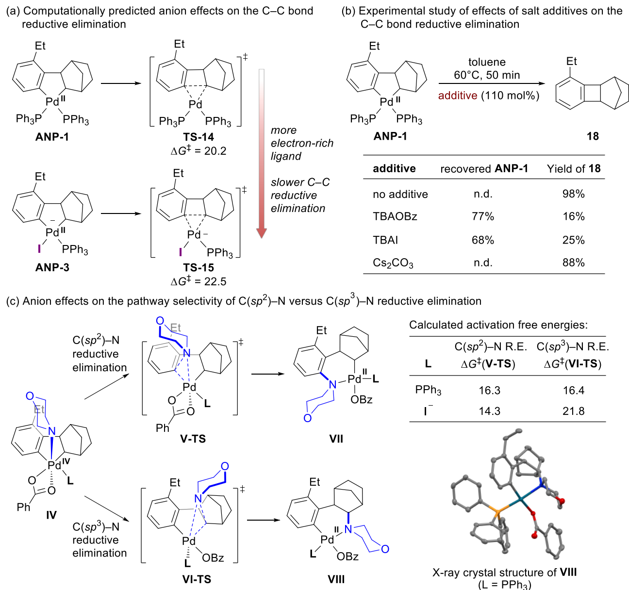
Fig. 4 Anion effects on the C–C bond reductive elimination and the pathway selectivity of C–N reductive elimination. All activation free energies are in kcal/mol with respect to the corresponding intermediate before the transition state.
