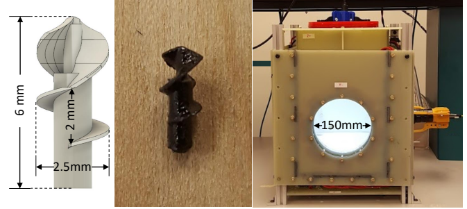
Fig. 2. CAD drawing (left) and picture of the helical swimmer (center). Picture of the magnetic manipulator used in this study (right).
