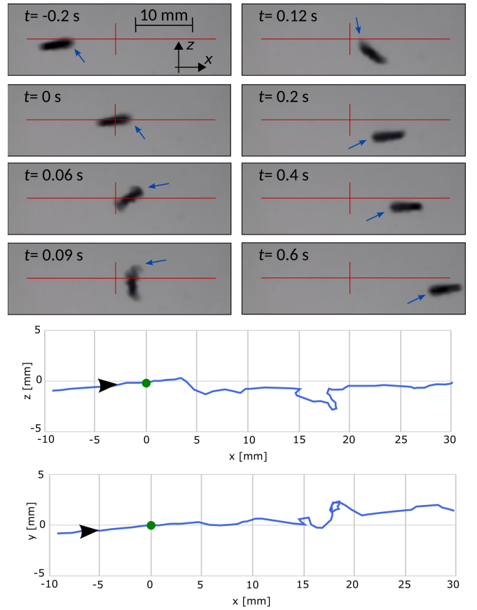
Fig. 9. Frames from the video and plot of the experimental trajectory obtained while performing an orientation reversal maneuver. The fore side of the swimmer is indicated by a blue arrow. The green dot indicates the position when the maneuver starts. The reference trajectory is z = y = 0 .
