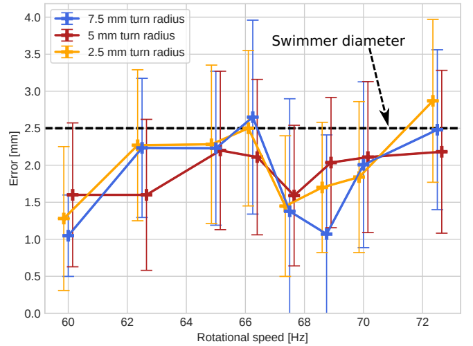
Fig. 5. The average swimmer position error while turning with radii of 7.5, 5 and 2.5 mm, is less than the swimmer diameter for all but two tests. Data points were recorded every 15 ms for 5 turns with each combination. The error bars represent the standard deviation of the measured data.
