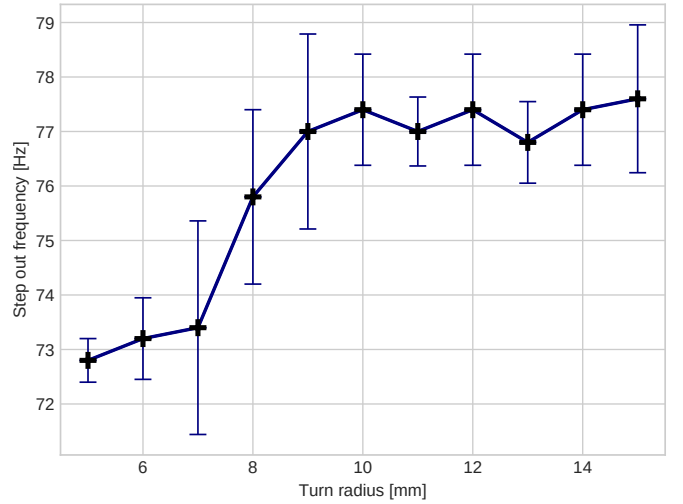
Fig. 7. Step-out frequency as a function of the turn radius for forward movement. Each data point represents five trials. The error bars represent the standard deviation of the measured data.
