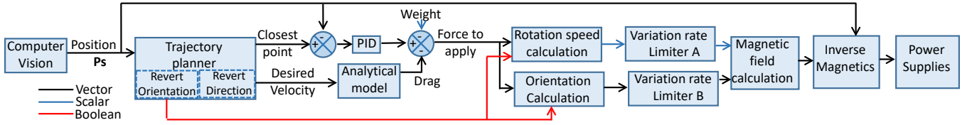
Fig. 3. Block diagram presenting the structure of the controller used in this study.
