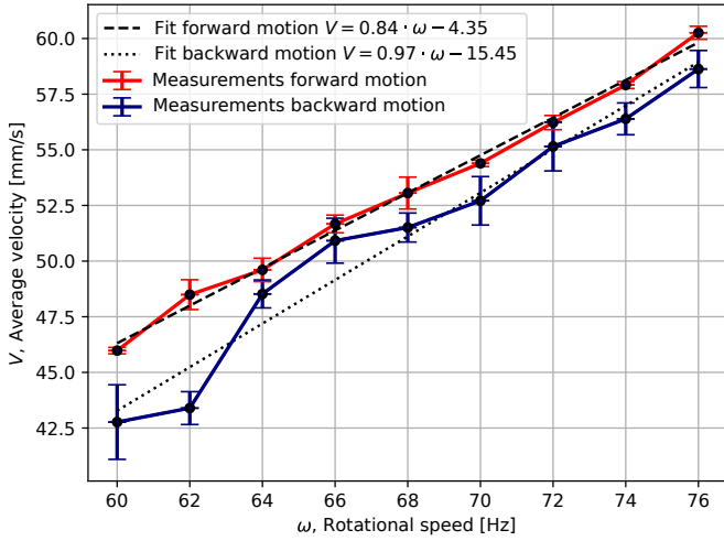
Fig. 6. Average velocity of the swimmer while performing a 180^\circ turn as a function of the rotational frequency. The turning radius was 7.5 mm. The forward and backward curves are approximated by the shown linear fits with coefficients of determination R^2_{\text{forward}}=0.995 and R^2_{\text{backward}}=0.96 .
