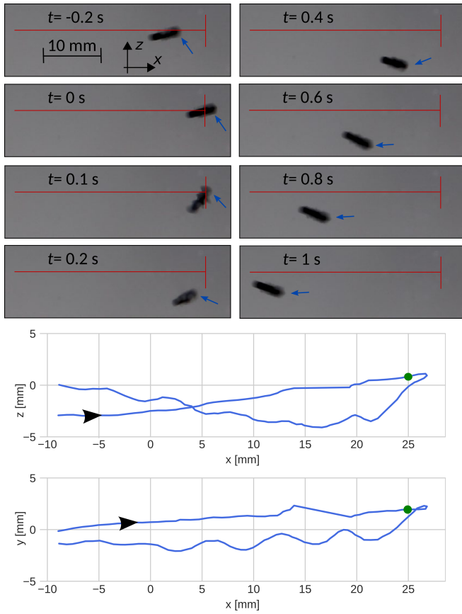
Fig. 8. Frames from the video and plot of the experimental trajectory obtained while performing a direction reversal maneuver. The fore side of the swimmer is indicated by a blue arrow. The green dot indicates the position when the maneuver starts. The reference trajectory is z = y = 0 .
