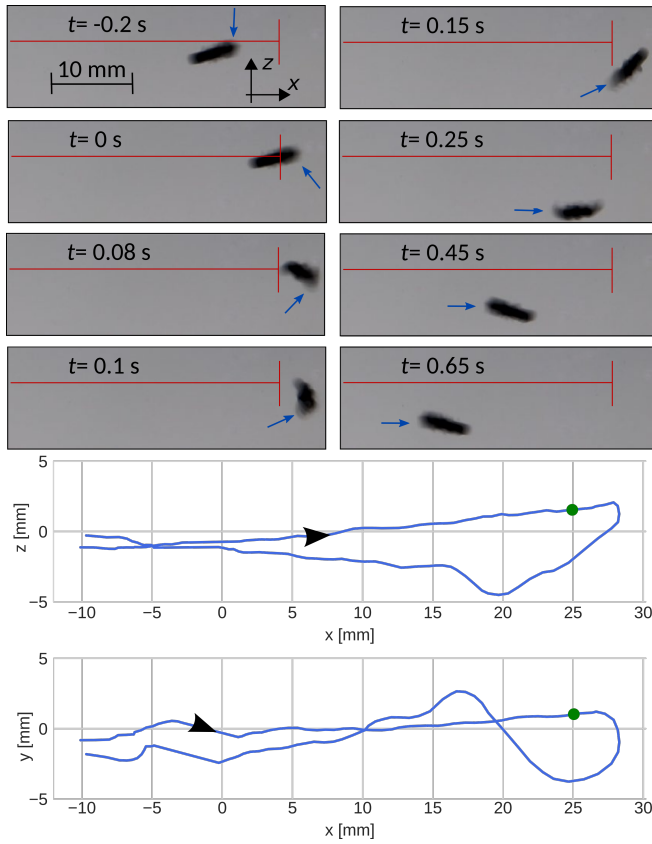
Fig. 10. Frames from the video and plot of the experimental trajectory obtained while performing a combined orientation and direction reversal maneuver. The fore side of the swimmer is indicated by a blue arrow. The green dot indicates the position when the maneuver starts. The reference trajectory is z = y = 0 .
