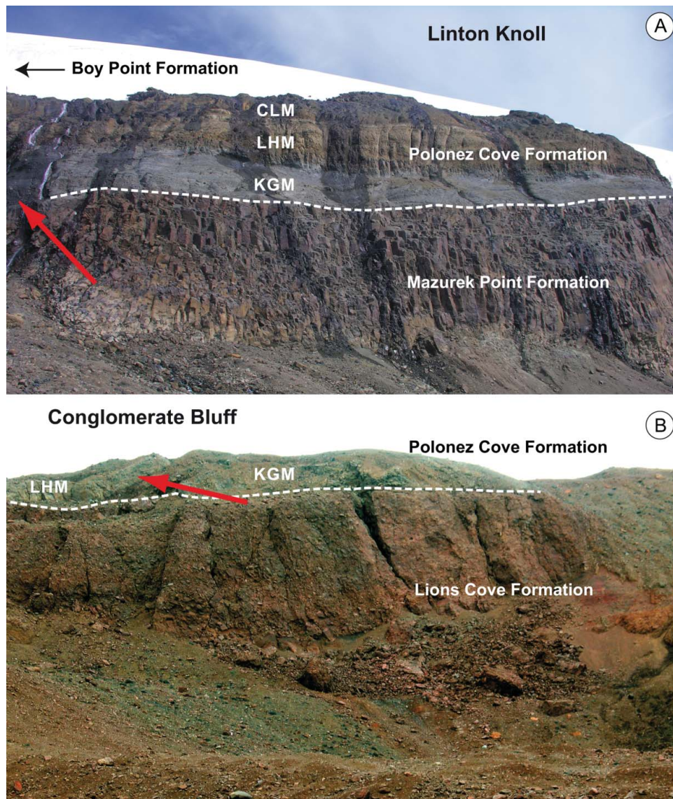
Figure 5. (A) Photograph of the section at Linton Knoll. (B) Photograph of the section at Conglomerate Bluff. King George Bay, King George Island. Red arrows indicate directions of the sections. KGM – Krakowiak Glacier Member; LHM – Low Head Member; CLM – Chlamys Ledge Member.
