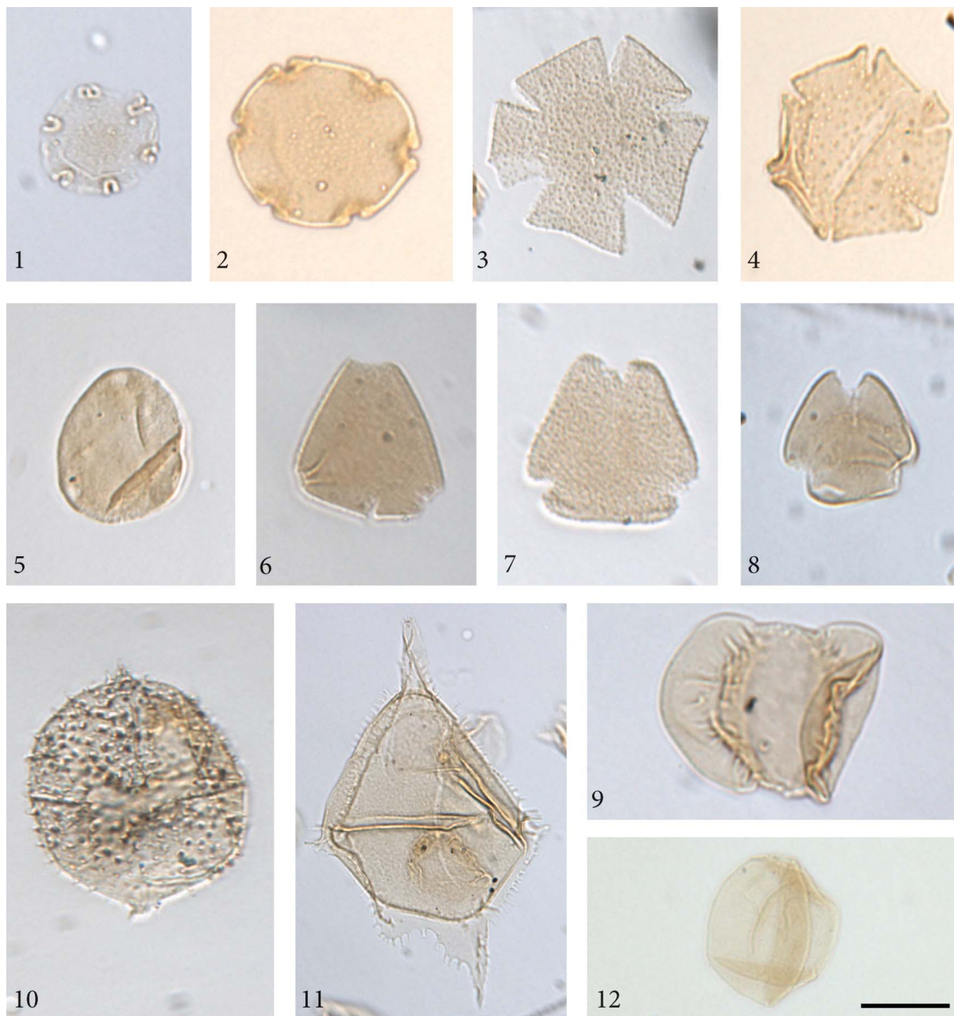
Plate 1. Light photomicrographs of palynomorphs considered in situ . Images 1–11 are from the La Meseta Fomation, Seymour Island, and 12 is from the Polonez Cove Formation, King George Island. 1–4. Various beech pollen grains: 1–2. Fusca group: Nothofagidites rocaensis-saraensis complex (1. sample D6-09 16.2 \times 139.1 ; 2 sample D6-08 15.9 \times 141.7 ); 3. Menziesii group: Nothofagidites sp. cf. N. asperus (sample D6-11 15.5 \times 117.5 ), 4. Brassii group: Nothofagidites mataurensis (sample D6-05 4.1 \times 143.5 ). 5–8. Other angiosperms: 5. Myricipites harrisii (sample D6-01 14.2 \times 119.4 ), 6. Proteacidites sp. cf. P. parvus (sample D6-01 13.4 \times 143.9 ), 7. Peninsulapollis askiniae (sample D6-03 16.2 \times 147.3 ), 8. Peninsulapollis gillii (sample D6-03 3.4 \times 144.4 ). 9. Gymnosperm: Phyllocladites sp. cf. P. exiguus (sample D6-08 13.3 \times 147.6 ). 10–12. Marine palynomorphs: 10. Vozzhennikovia rotunda (sample D6-01 6.3 \times 117.8 ), 11. Spinidinium macmurdoense (sample D6-12 14.6 \times 144.9 ), 12. Leiosphaeridia sp. (Sample G-13 12.1 \times 141.0 ). All images were taken at 60\times under oil immersion. Scale bar = 20\ \mu\text{m} .
