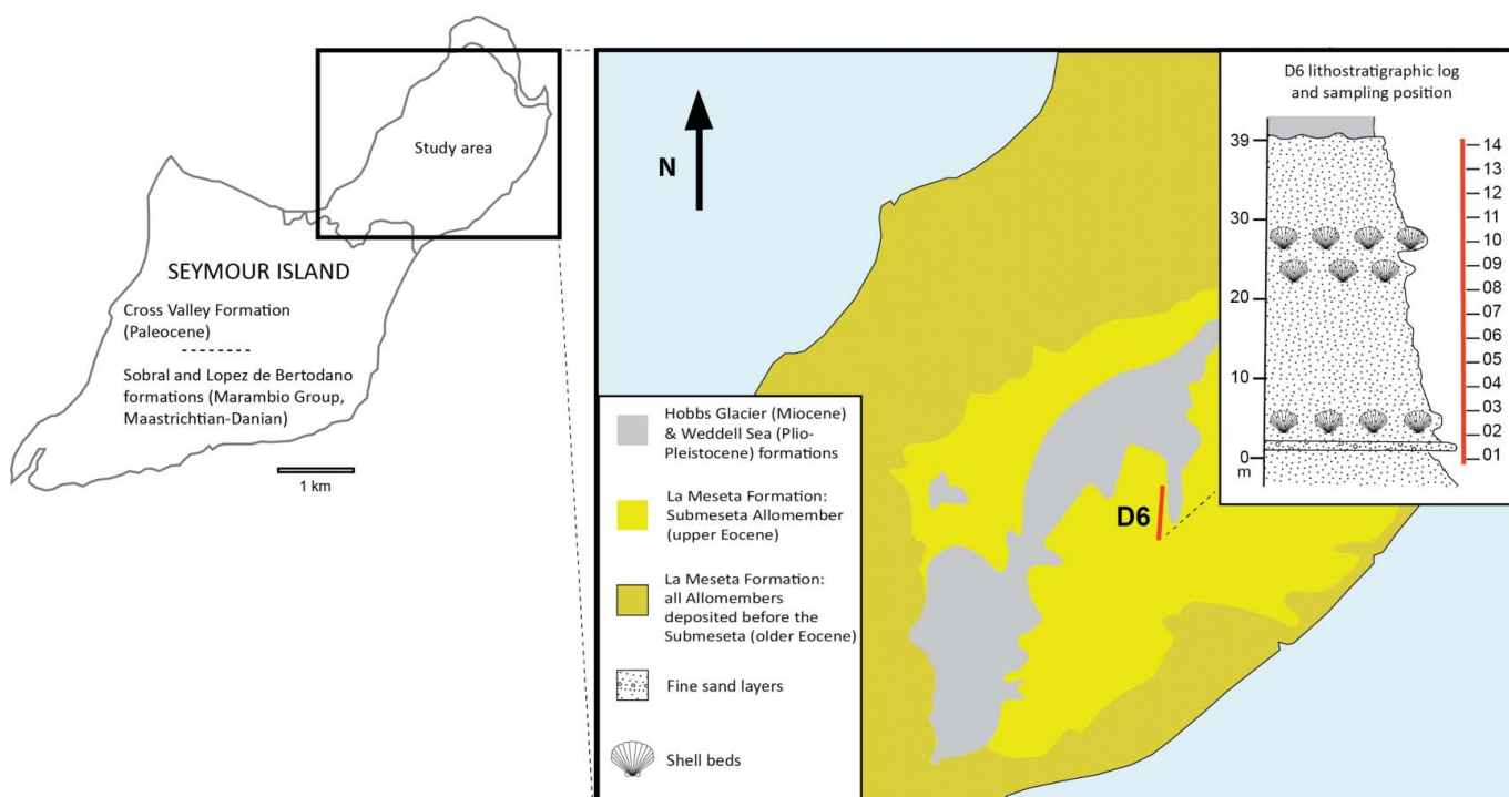
Figure 2. Simplified geological map of northern Seymour Island, showing the La Meseta Formation with the distribution of the Submeseta Allomember in relationship to other La Meseta allomembers. The location of the D6 section is marked by a red line. The relationship of the sample location with the lithology sampled is presented in the inset to the right.
