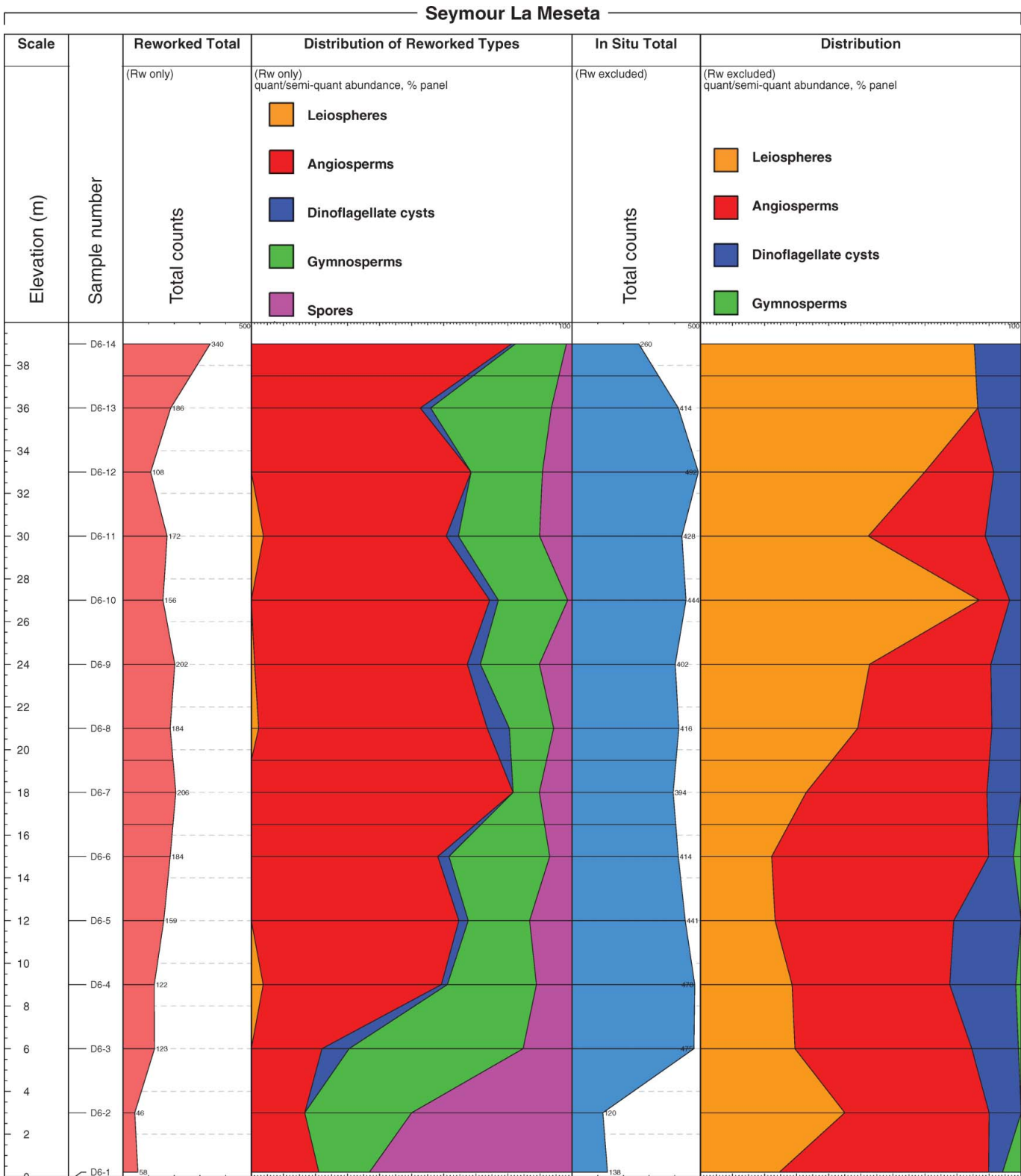
Figure 8. Relative abundance of reworked (Rw) and in situ palynomorphs in La Meseta Formation samples.
