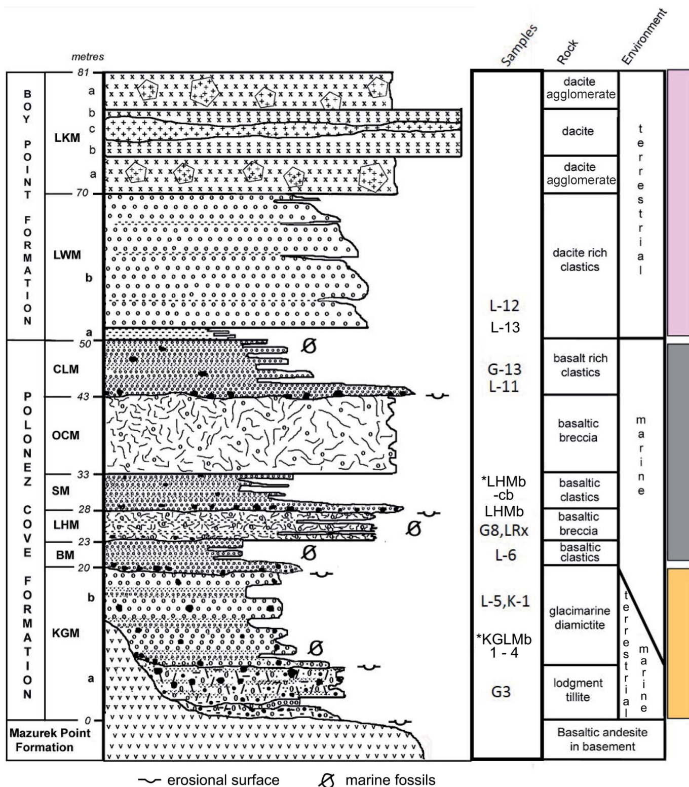
Figure 6. Detailed section of the Polonez Cove Formation at Linton Knoll showing samples collected during the PAS expeditions in 2007 and 2009. * indicates stratigraphic location of samples from the adjacent Conglomerate Bluff section. Polonez Cove Formation: KGM – Krakowiak Glacier Member; BM – Bayview Member; LHM – Low Head Member; SM – Siklawa Member; OCM – Oberek Member; CLM – Chlamys Ledge Member. Boy Point (BP) Formation: LWM – Loud Waterfall member; LKM – Linton Knoll member.
