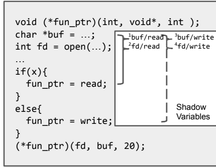
Figure 3: For function pointer arguments, dynamic binding creates shadow copies for every pair of originating variable and target function. Here, read and write are both possible targets of fun_ptr , and the buf and fd variables are both passed as arguments, resulting in four different shadow variables, one for each pair.
