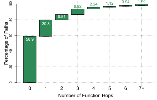
Figure 6: Cumulative distribution of the number of caller functions traversed during backward analysis for reaching the definition of protected arguments. More than half of the arguments are found within the same function.
