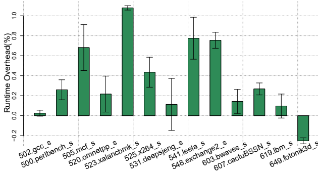
Figure 5: Saffire’s runtime overhead for the SPEC2017 benchmarks with all libc functions instrumented. The average overhead across all benchmarks was 0.34%.
