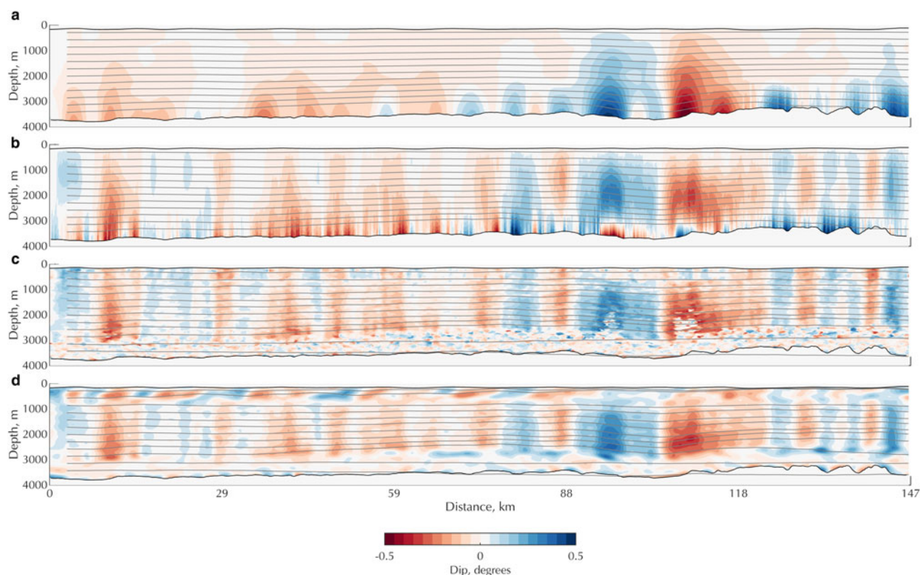
Fig. 3. Propagation of a streamline through dip fields derived from (a) reference picks, (b) Panton slope-extraction step, (c) ARES and (d) using PWD.
