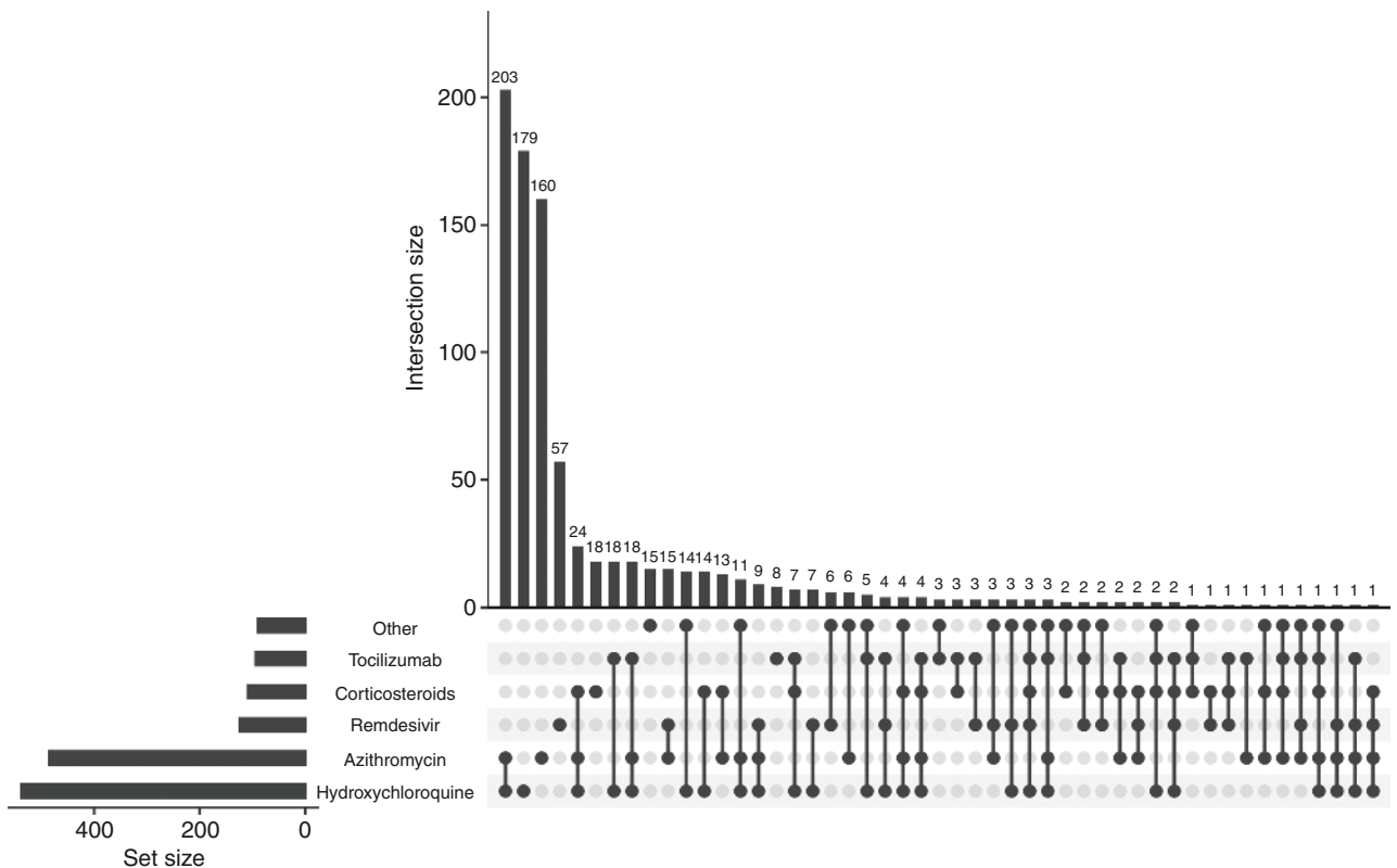
Figure 3. UpSet plot of treatment exposures. There are a total of 865 treatment exposures observed across 49 different patterns.
