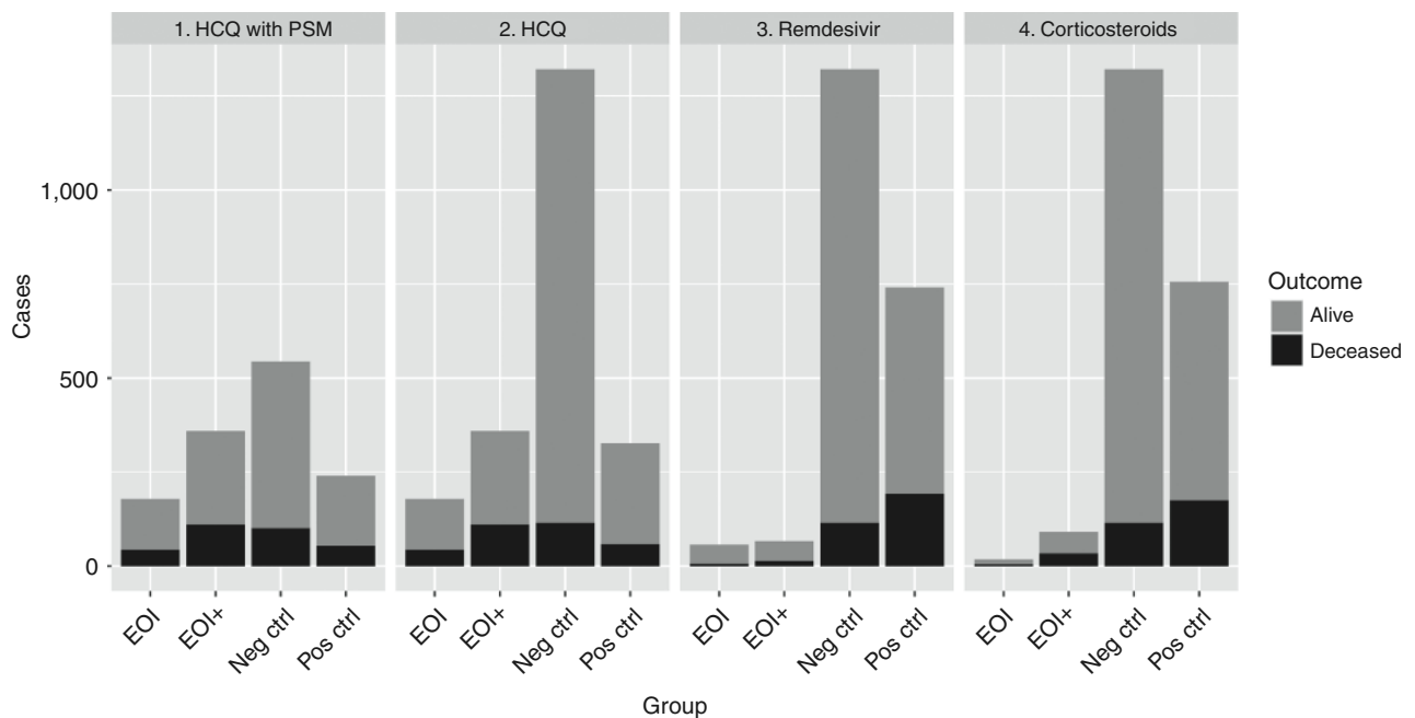
Figure 4. Distribution of matched and unmatched cohorts stratified by exposure of interest (EOI). Negative controls are patients who did not have any reported COVID-19 treatment; positive controls are patients who had a treatment reported that did not include the EOI. EOI+, EOI with any other exposure; HCQ, hydroxychloroquine.
