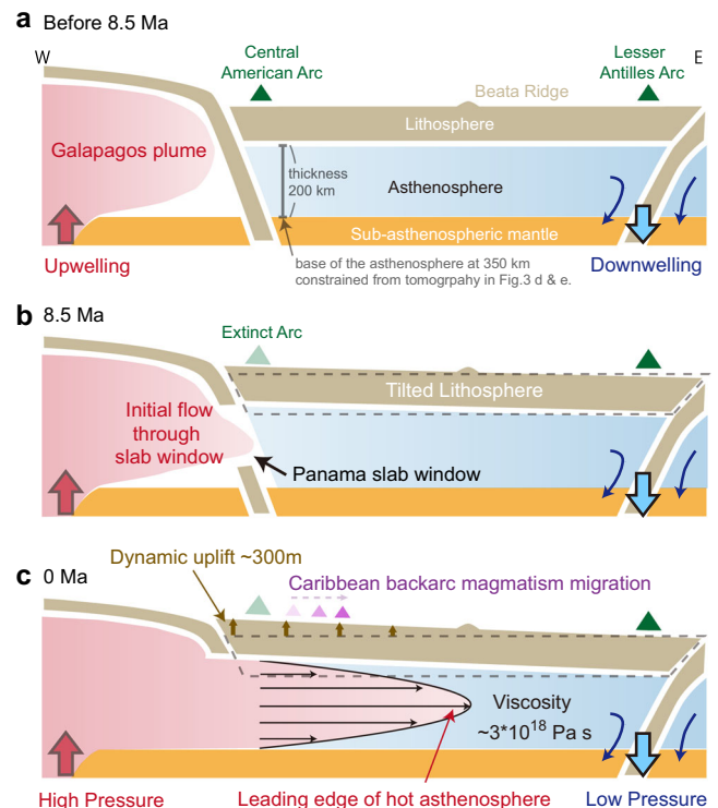
Fig. 5 Time-evolution cartoon of Caribbean asthenosphere and dynamic topography. Hotter asthenosphere sourced from the Galapagos plume flowed eastwards through the Central America slab window towards the Caribbean and produced an eastward dynamic tilt of the Earth's surface.
