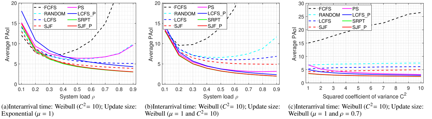
Fig. 17: Comparisons of the average PAoI performances of several common scheduling policies under different distributions
