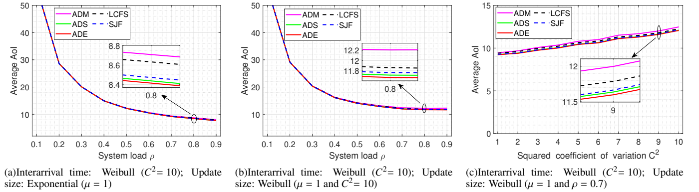
Fig. 18: Comparisons of the average AoI performance under different distributions: AoI-based policies vs. non-AoI-based policies
