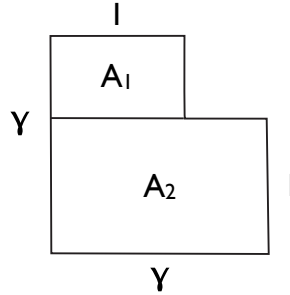
Figure 2. The golden table P .
