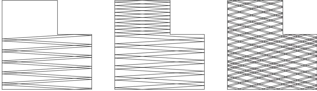
Figure 1. Periodic billiard trajectories with slopes tending to zero.
