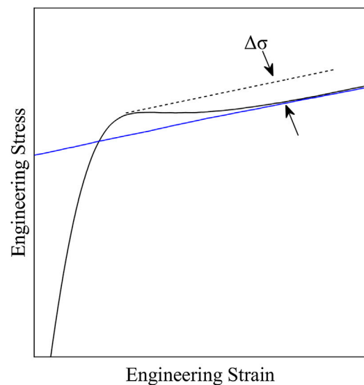
FIGURE 4 | Change in yielding ( \Delta\sigma ), shown as the difference between the upper yield point and the stress at the strain of the maximum yield assuming the work hardening rate of the sample after yielding.
