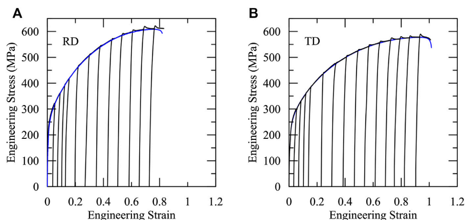
FIGURE 2 | Engineering stress vs engineering strain of a 304 stainless-steel in the (A) rolling direction and (B) transverse direction from monotonic and interrupted tests. Tests were performed at room temperature and a strain rate of 0.001 \text{ s}^{-1} . The interrupted tests were fully unloaded and held at room temperature prior to reloading.
