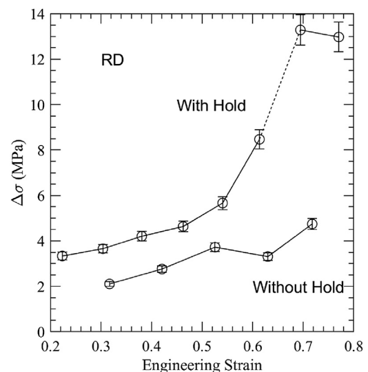
FIGURE 5 | Change in yielding of a 304 stainless steel during interrupted tensile testing performed at room temperature and a strain rate of 0.001 \text{ s}^{-1} , with and without an isothermal hold between straining steps.
