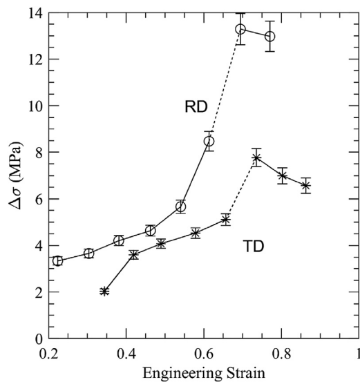
FIGURE 3 | Change in yielding ( \Delta\sigma ) after an isothermal 2 h hold at room temperature of a 304 stainless steel in the rolling direction and transverse direction during interrupted tensile tests performed at room temperature and a strain rate of 0.001 \text{ s}^{-1} . The maximum seen at a strain of \sim 0.7 strain corresponds to an extended isothermal hold at room temperature.
