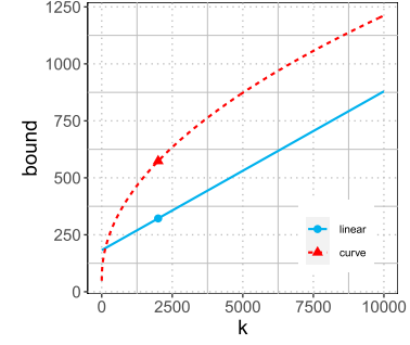
(b) Plot of two bounds. The linear bound ( m = n/4 ) is tighter for most k \leq 10^4 .
