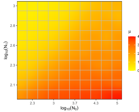
FIG 2. Sufficient signal strength \mu for AMT to guarantee both type-I and type-II error control at 0.05 (derived from (12)), when varying the numbers of nulls N_0 \in [10^2, 10^5] and non-nulls N_1 \in [10^2, 10^3] . The required signal strength grows when the number of nulls increases or the number of non-nulls decreases.
