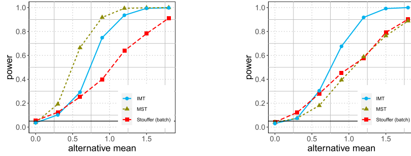
(a) The power against non-null signal. The non-null block is in the grid center. (b) The power against non-null signal. The non-null block is in the grid corner.
