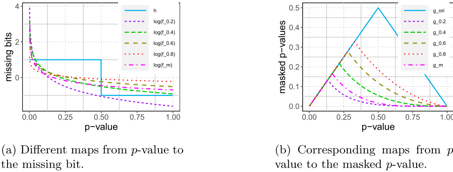
FIG 10. Different choices of missing bit and its corresponding masked p -value. When small p -values (possible non-nulls) are more evident when measured by one choice of the missing bit, they are less distinctive when looking at the corresponding masked p -values.
