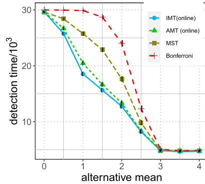
FIG 7. Number of hypotheses needed to reject the global null (detection time) in the online setting of the interactively ordered martingale test (IMT), the adaptively ordered martingale test (AMT), the martingale Stouffer test (MST), and the Bonferroni test when varying the alternative mean \mu . The non-nulls arrive in blocks, and on average, every 10^4 hypotheses contain a block of 500 non-nulls. The length of the error bar is two standard error. The interactively ordered martingale test is the first to reject the global null because it incorporates the block structure and adjusts the discarding threshold based on past p -values.
