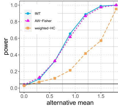
FIG 16. Power of the interactively ordered martingale test (IMT), AW-Fisher, and weighted-HC when the non-null cluster is in the center of a 10 \times 10 grid. IMT and AW-Fisher both have high power, but the AW-Fisher has a high computational cost.
