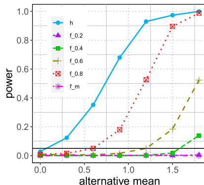
FIG 11. Power of interactive tests using different missing bits. Under the block structure of non-nulls as described in Section 5.1, the IMT with the original missing bit defined in equation (3) has the highest power.
