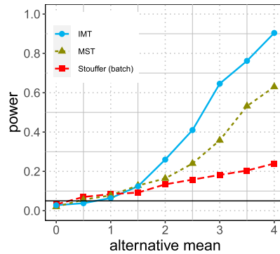
FIG 5. Power of the interactively ordered martingale test (IMT), the martingale Stouffer test (MST), and the batch Stouffer test under a hierarchical structure. Hypotheses form a fixed tree (batch setting) with non-nulls only on a sub-tree. When the alternative mean is big, masked p -values and the hierarchical non-null structure lead to a good ordering and hence high power for the IMT.
