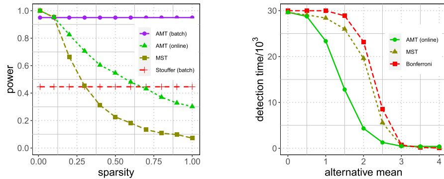
(a) Power comparison in the batch setting when varying the prior ordering. Larger sparsity indicates a worse prior ordering. The AMT procedures (batch and online) adaptively alter the ordering and are more robust to bad quality of orderings than MST. Still, when the prior ordering is great, AMT has lower power than MST because the increments of AMT's test statistic are bounded by +1 . This phenomenon is mathematically predicted by Theorem 4 and Theorem 5.
