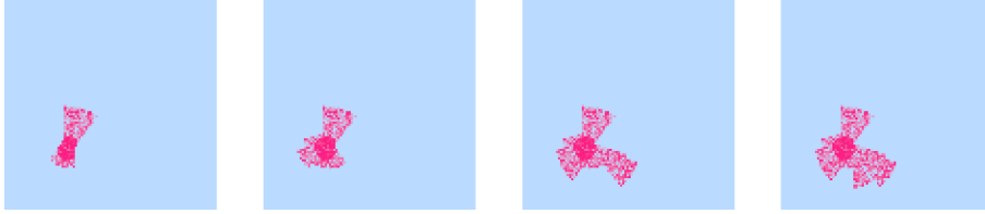
FIG 3. Visualization of the interactively ordered martingale test under the block structure: the hypotheses in M_k , which interactively expands (darker color indicates a lower p -value and possible non-null).
