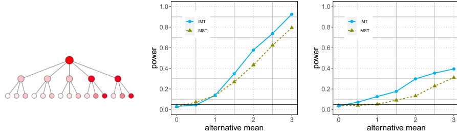
(a) Hypothesis tree with decreasing non-null probability, which is marked by fading red nodes. (b) Power against alternative mean in a hypothesis tree with decreasing probability of being non-null. (c) Power against alternative mean in a hypothesis tree with increasing probability of being non-null.
