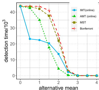
FIG 8. Number of hypotheses needed to reject the global null (detection time) in the online setting of the interactively ordered martingale test (IMT), the adaptively ordered martingale test (AMT), the martingale Stouffer test (MST), and the Bonferroni test when varying the alternative mean in a growing hypothesis tree (online setting). IMT incorporates the hierarchical structure of non-nulls, so it is the first to reject the global null when the non-null signal is mild ( \mu < 2 ).
