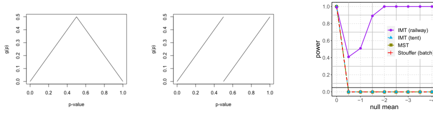
(a) The original masking function (tent). (b) The modified masking function (railway). (c) Power when varying the null means (negative values indicate conservative nulls).
