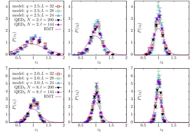
FIG. 4. Distribution of scaled eigenvalues z_i = (\Lambda_i/\langle\Lambda_i\rangle) for the three lowest eigenvalues (left to right) from the conformal lattice model at q = 2.5 (top) and q = 2.0 (bottom) are compared with those from N = 2 and N = 8 QED 3 . For the lattice model, results from L = 24, 28, 32 are shown, where as for QED 3 , results from two large box sizes \ell (measured in units of coupling g^2 ) are shown.
