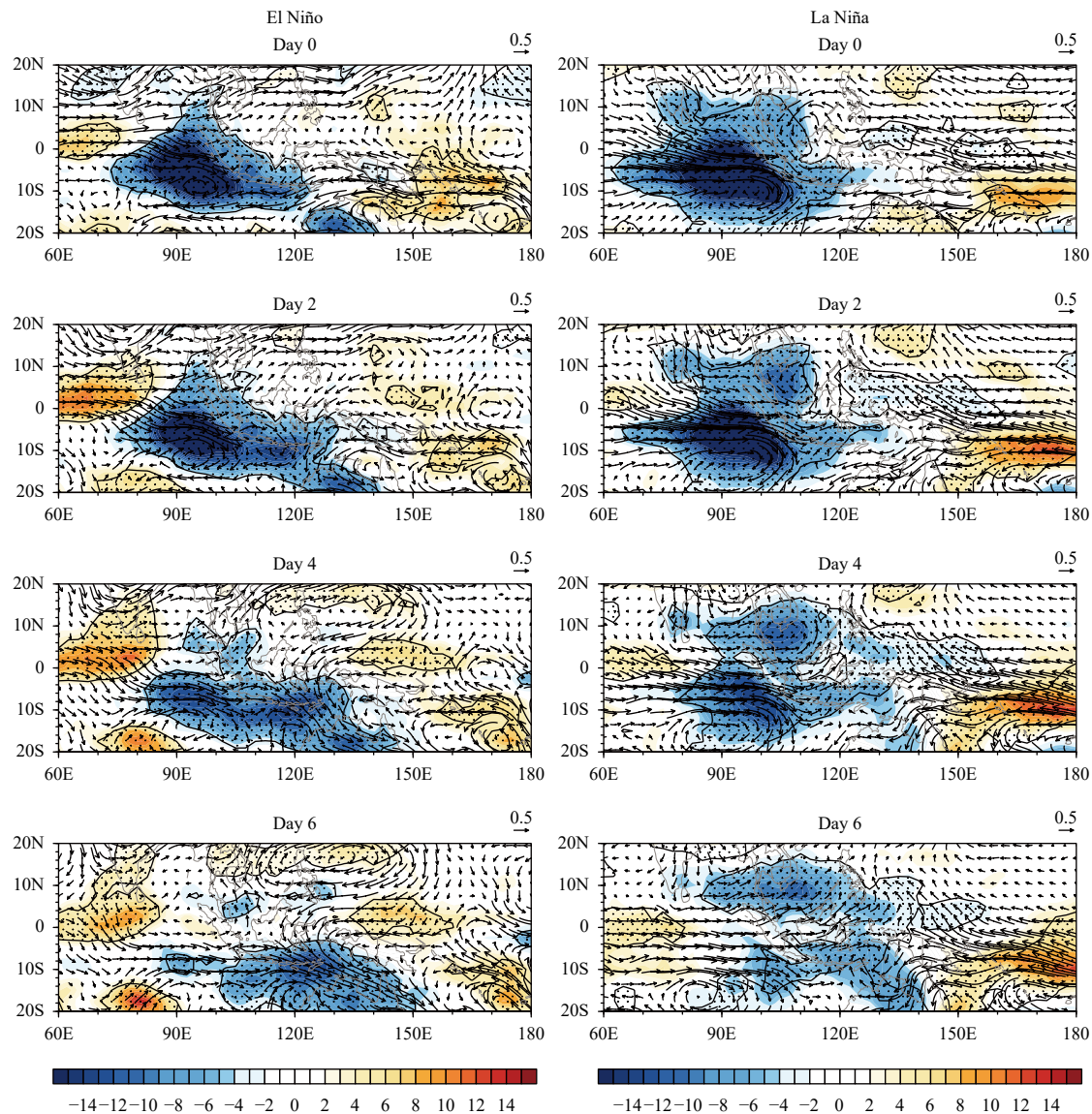
Fig. 2. Lead-lag regressed patterns of 10–90-day filtered OLR anomaly (shaded; \text{W m}^{-2} ) and associated wind anomaly field at 850 hPa (vector; \text{m s}^{-1} ) from Days 0 to 6. The regression was based on the OLR anomaly at a reference point over Indian Ocean ( 5^{\circ}\text{S} , 95^{\circ}\text{E} ) for EP El Niño (left) and La Niña (right) winters. The OLR anomalies that pass the significant test at 95% confidence level are stippled.
