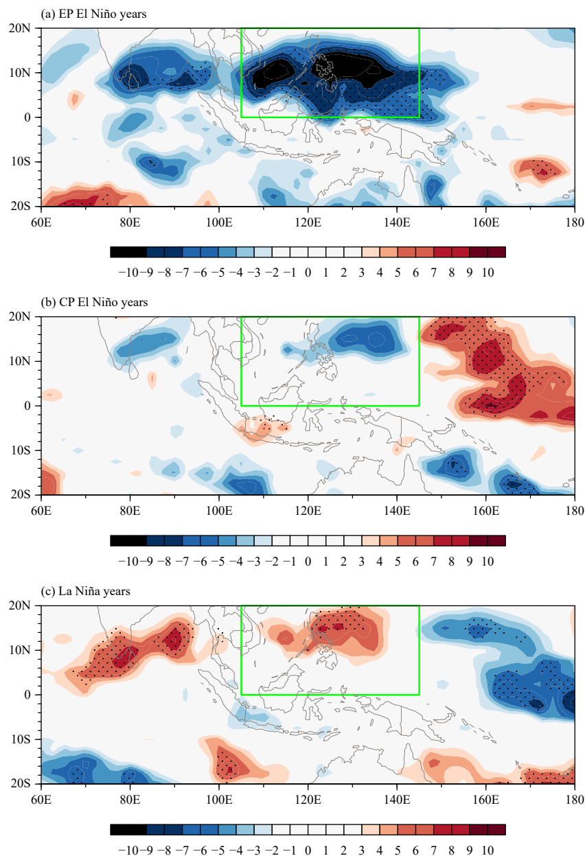
Fig. 1. Standard deviation (STD) of 10–90-day band-pass filtered OLR anomalies (shaded; \text{W m}^{-2} ) for (a) EP El Niño, (b) CP El Niño, and (c) La Niña. Climatological STD at each grid point has been subtracted at each panel. The green box denotes a key region ( 0^{\circ} – 20^{\circ}\text{N} , 105^{\circ} – 145^{\circ}\text{E} ) where ENSO exerts a strong impact on MJO.
