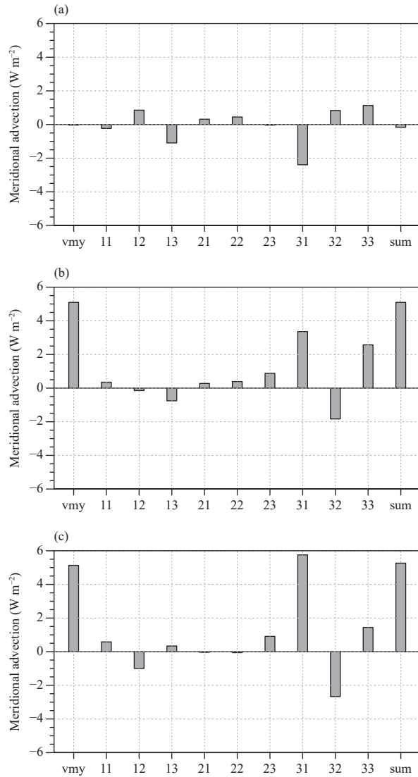
Fig. 11. Decomposition of the anomalous meridional MSE advection term ( -\langle v \partial m / \partial y \rangle' ; \text{W m}^{-2} ) averaged over the northern box (red box in Fig. 8) for (a) EP El Niño, (b) La Niña, and (c) their difference (La Niña minus EP El Niño). Bars from left to right represent total and each component of the meridional advection term: -\langle v \partial m / \partial y \rangle' , -\langle v_1 \partial m_1 / \partial y \rangle' , -\langle v_1 \partial m_2 / \partial y \rangle' , -\langle v_1 \partial m_3 / \partial y \rangle' , -\langle v_2 \partial m_1 / \partial y \rangle' , -\langle v_2 \partial m_2 / \partial y \rangle' , -\langle v_2 \partial m_3 / \partial y \rangle' , -\langle v_3 \partial m_1 / \partial y \rangle' , -\langle v_3 \partial m_2 / \partial y \rangle' , -\langle v_3 \partial m_3 / \partial y \rangle' , and the sum of the nine decomposed terms. Here subscripts 1, 2, and 3 denote the climatological annual cycle, interannual, and high frequency ( < 90 days) components.
