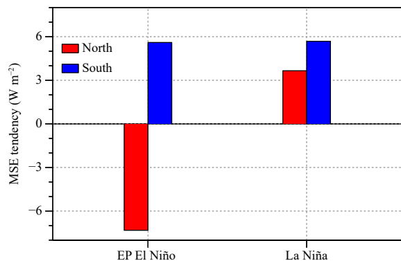
Fig. 9. MSE tendency ( \text{W m}^{-2} ) anomalies averaged over the northern (red) and southern (blue) boxes shown in Fig. 8 for EP El Niño (left) and La Niña (right).
