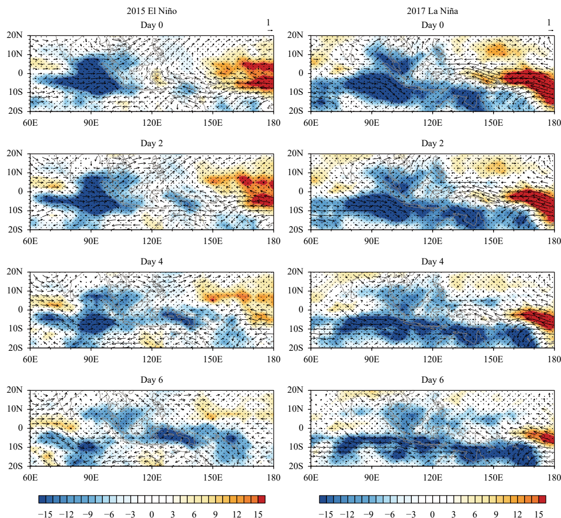
Fig. 15. Lead-lag regressed patterns of 10–90-day filtered OLR anomaly (shaded; \text{W m}^{-2} ) and associated wind anomaly field at 850 hPa (vector; \text{m s}^{-1} ) from Days 0 to 6. The regression was based on the OLR anomaly at a reference point over Indian Ocean ( 5^{\circ}\text{S} , 95^{\circ}\text{E} ) during 2015 El Niño (left) and 2017 La Niña (right) winter (DJF), respectively. The OLR anomalies that pass the significant test at 95% confidence level are stippled.
