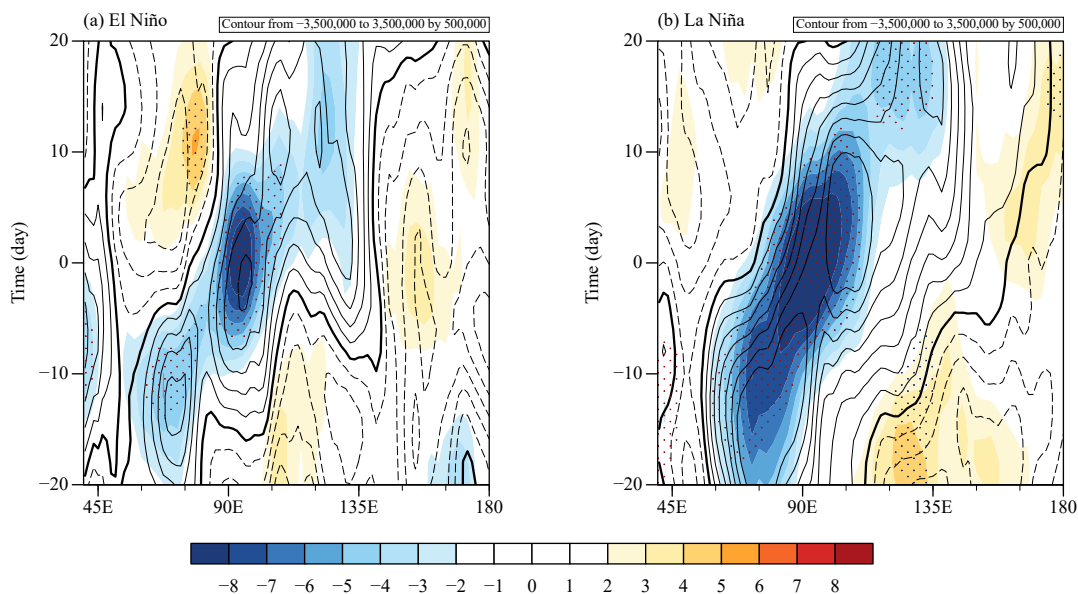
Fig. 3. The Hovmöller diagram of the regressed OLR (shaded; \text{W m}^{-2} ) and column-integrated MSE (contour; \text{J m}^{-2} ) anomalies averaged over 20^{\circ}\text{S} – 20^{\circ}\text{N} for (a) EP El Niño and (b) La Niña winters from Days –20 to 20. The regression was based on the OLR anomaly at 5^{\circ}\text{S} , 95^{\circ}\text{E} . The OLR anomalies that pass the significant test at 95% confidence level are stippled.
