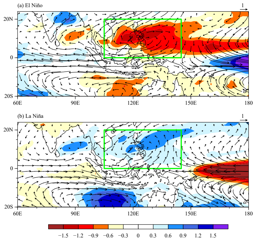
Fig. 4. Background specific humidity (shaded; \text{g kg}^{-1} ) and 850-hPa wind (vector; \text{m s}^{-1} ) fields during (a) El Niño and (b) La Niña winters (DJF). Climatological mean specific humidity and 850-hPa wind fields have been subtracted at each panel. The green box shows the same region as that in Fig. 1.
