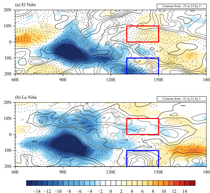
Fig. 8. Horizontal patterns of the OLR anomaly (shaded; \text{W m}^{-2} ) and column-integrated MSE tendency (contour; \text{W m}^{-2} ) fields regressed onto the OLR anomaly at the reference point (5°S, 95°E) for EP El Niño (top) and La Niña (bottom) winters. The red and blue boxes are key regions for the MSE budget analysis in front of the MJO convection.
