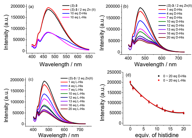
Figure 1. Fluorescence spectra of ( S )- 3 (0.01 mM) + Zn(OAc) 2 (2.0 equiv) with (a) D- and L-histidine (10.0 equiv), (b) D-histidine, and (c) L-histidine. (d) Fluorescence intensity at 470 nm versus the equivalence of D- and L-histidine (Error bars from three independent experiments. \lambda_{\text{exc}} = 378 nm. Slit: 5/5 nm. Solvent: DMF/1% pH 6.35 phosphate buffer)
