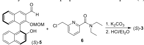
Scheme 3. Synthesis of the proposed fluorescent probe ( S )- 3
