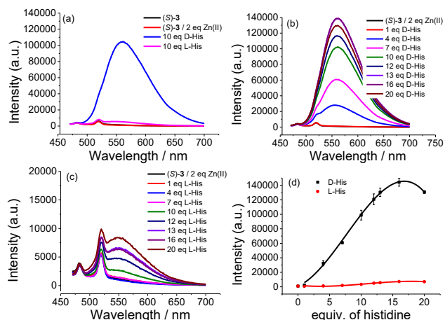
Figure 2. Fluorescence spectra of ( S )- 3 (0.01 mM) + Zn(OAc) 2 (2.0 equiv) with (a) D- and L-histidine (10.0 equiv), (b) D-histidine, and (c) L-histidine. (d) Fluorescence intensity at 560 nm versus the equivalence of D- and L-histidine (Error bars from three independent experiments. \lambda_{\text{exc}} = 450 nm. Slit: 5/5 nm. Solvent: DMF/1% pH 6.35 phosphate buffer)
