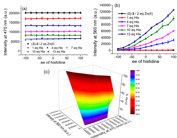
Figure 5. Fluorescence response of ( S )- 3 (0.01 Mm) + Zn(OAc) 2 (2.0 equiv) toward histidine (0 - 13 equiv). (a) I_{470} ( \lambda_{\text{exc}} = 378 nm) versus ee of histidine at varying concentration. (b) I_{560} ( \lambda_{\text{exc}} = 450 nm) versus ee of histidine at varying concentration. (c) I_{470} versus I_{560} at varying [D-His]%. (Solvent: DMF/1% pH 6.35 phosphate buffer. All the data were obtained from three independent experiments. Slit: 5/5 nm)
