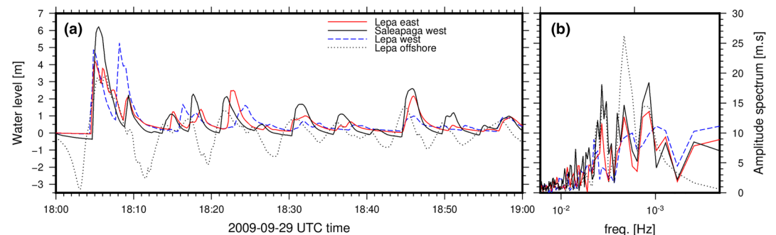
Figure 7. (a) Time series of water level for scenario Lay et al. (2010) Version C showing the variability of onshore hydrodynamics response at Lepa and Salepaga, and offshore of Lepa. (b) Amplitude spectrum showing local variability of onshore and offshore wave energy and excitation frequencies.
