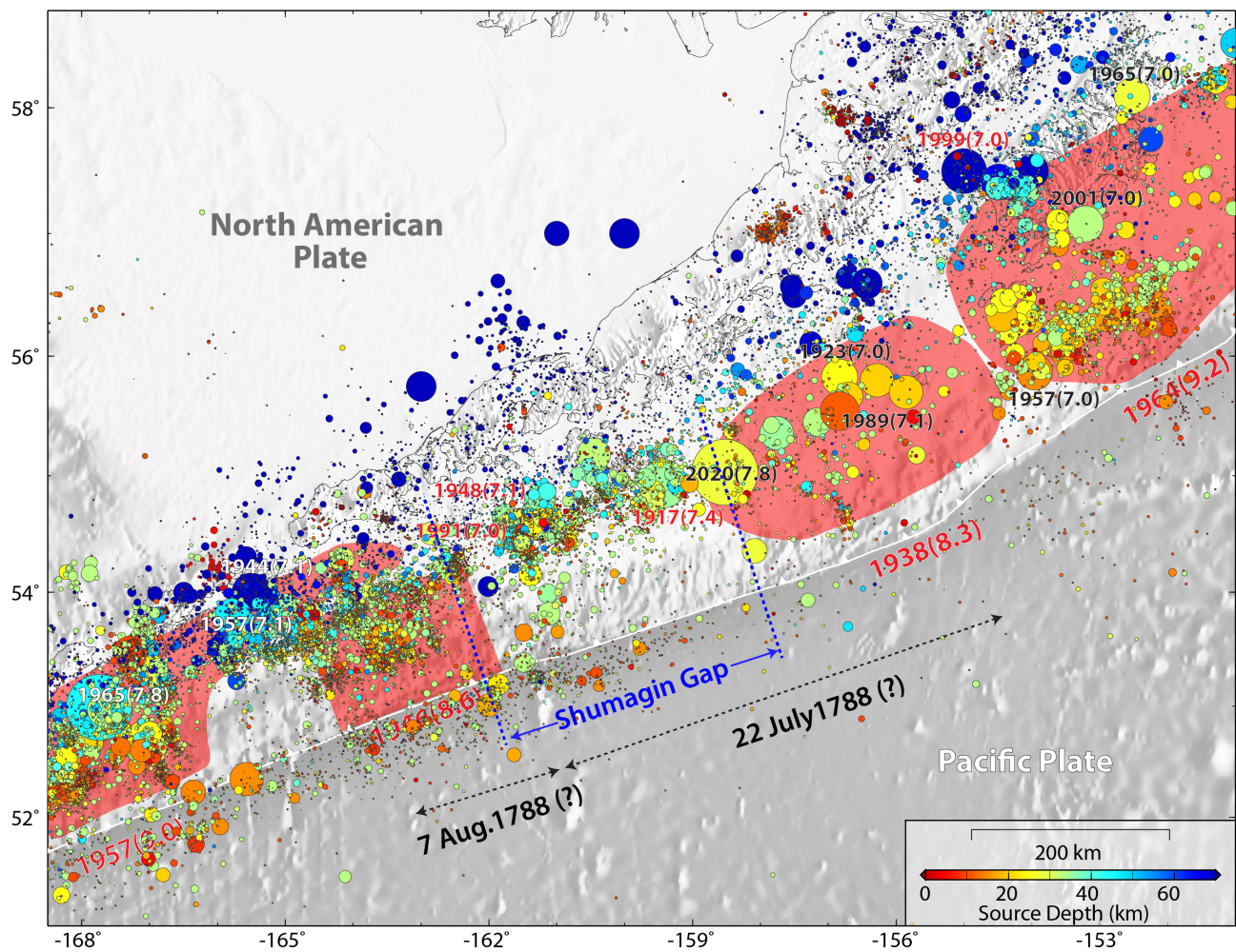
Figure S1. Seismicity around the 2020 Shumagin, Alaska earthquake since 1900 from the USGS-NEIC catalog, color-coded with their source depth. The radius of each circle is proportional to the event magnitude. Year and magnitude of events with M \geq 7.0 are labeled.
