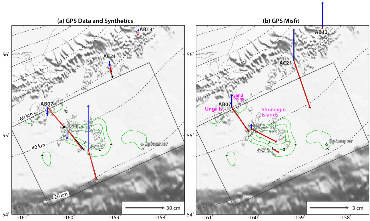
Figure S3. GPS misfit with the preferred slip model for the 2020 M_w 7.8 Alaska earthquake. (a) GPS data (black) and synthetics. Vertical and horizontal vectors show the vertical and horizontal displacements, respectively. Blue and red vectors show predicted vertical and horizontal displacement from the preferred slip model. (b) Vertical (blue) and horizontal (red) residual displacements (data minus synthetics). Green contours in (a) and (b) show the surface projection of 1-m slip contours for the M_w 7.8 mainshock.
