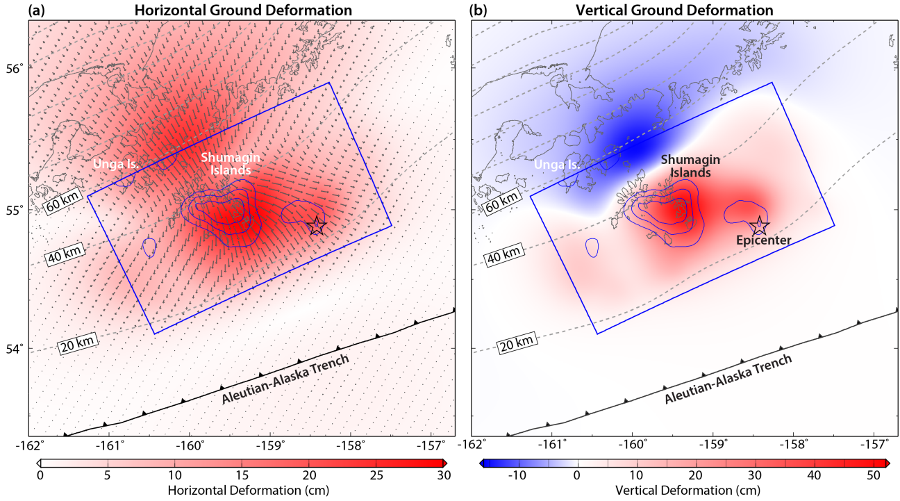
Figure S5. Ground deformation from the preferred slip model for the 2020 M_W 7.8 Alaska earthquake. (a) Horizontal deformation with arrows indicating deformation directions. (b) the vertical deformation. The blue box in (a) and (b) shows the surface projection of the rupture plane for the M_W 7.8 mainshock along with 1-m slip contours (blue). The gray-dashed curves in both (a) and (b) are 20 km depth contours of the slab interface from model Slab2 (Hayes et al., 2018).
