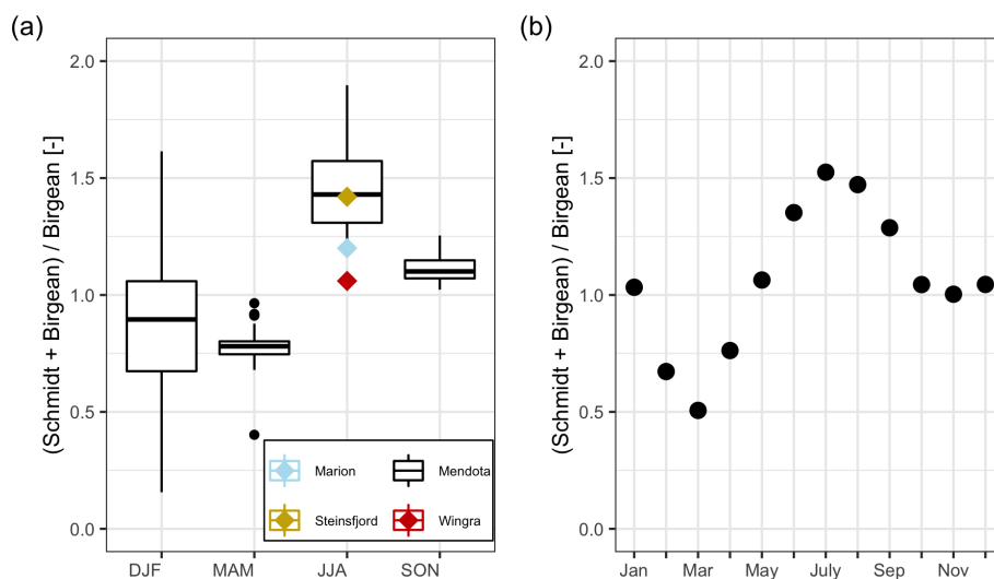
Figure 7. Dynamics of the average HBR = (St + B) / B over time. (a) Boxplots of the HBR over the meteorological seasons, which represent seasonal quarters of the year beginning in December. The summer HBR values for Lake Marion, Lake Steinsfjord, and Lake Wingra were taken from Kjensmo (1994). (b) Scatterplot of the average HBR values for each month.
