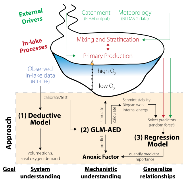
Figure 2. Schematic overview of the modeling workflow: (1) application of a deductive model to further our system understanding about oxygen sink terms; (2) replication of Lake Mendota using GLM-AED2 to investigate hydrodynamic and ecosystem mechanisms; and (3) application of regression models to quantify the importance of ecosystem predictors on the anoxic factor.
