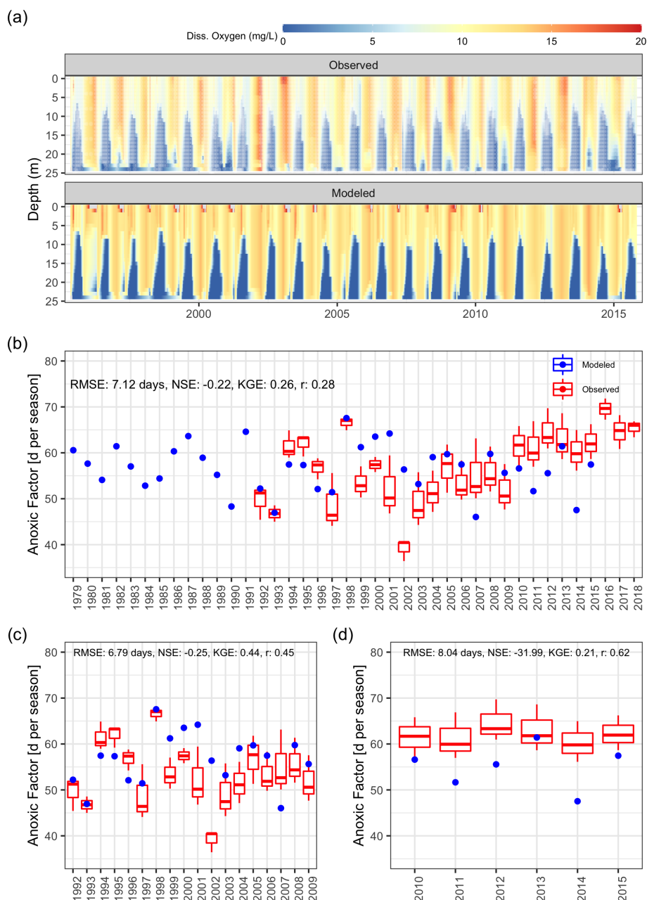
Figure 10. Comparison of observations to GLM-AED modeled dissolved oxygen concentrations and ecosystem response. (a) Contour plot of observed (upper figure, white dots mark sample events) and simulated dissolved oxygen concentrations. (b) Comparison of simulated anoxic factor (blue dots) against interpolated range of anoxic factor derived from observed data (box-whisker plots) over the period 1979 to 2018. (c) Comparison of simulated anoxic factor (red dots) against interpolated range of anoxic factor derived from observed data (box-whisker plots) over the period 1992 to 2009. (d) Comparison of simulated anoxic factor (red dots) against interpolated range of anoxic factor derived from observed data (box-whisker plots) over the period 2010 to 2015.
