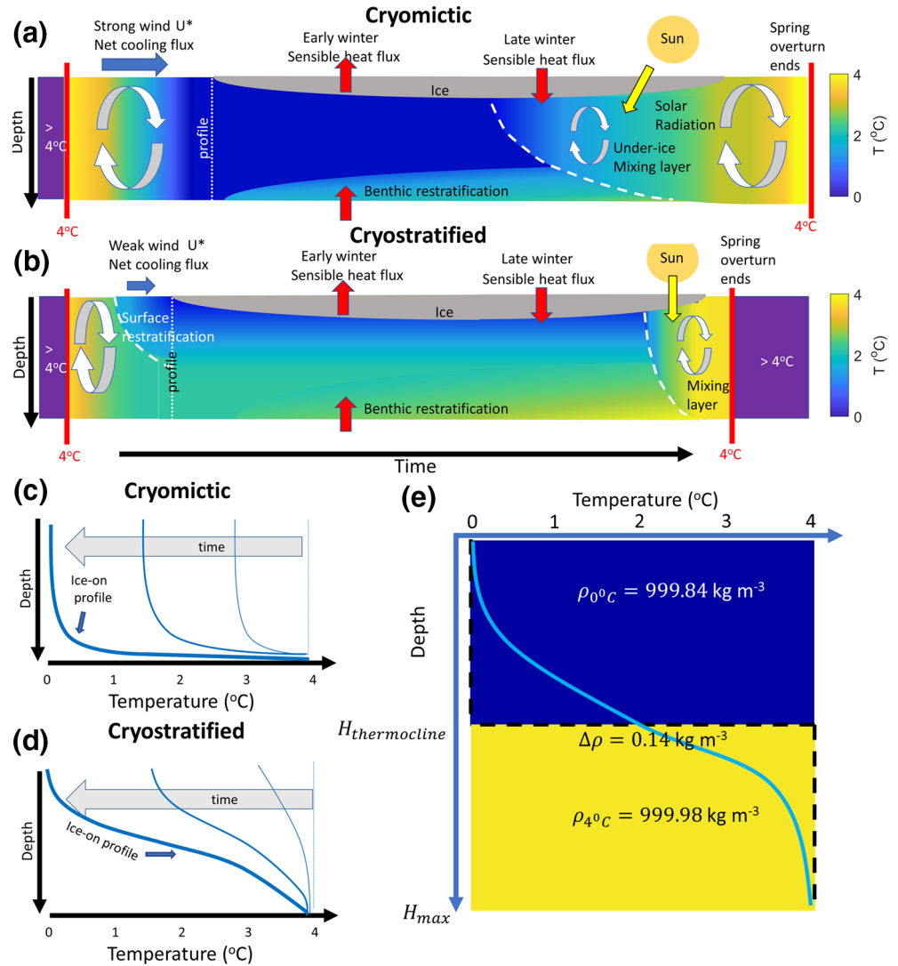
Figure 1. Schematic showing the difference in thermal structure between (a) a wide, shallow, and windy lake with a deeper cold layer and weak stratification, and (b) a small, deep, and calm lake with strong inverse stratification. Corresponding evolution of temperature profiles until ice-on for (c) wide lake and (d) small lake. (e) An idealized schematic of winter thermocline depth H_{thermocline} used to develop our theory with the black dashed line showing the vertical temperature profile for the idealized two-layer model and the blue curve as an example of an actual vertical temperature profile.
