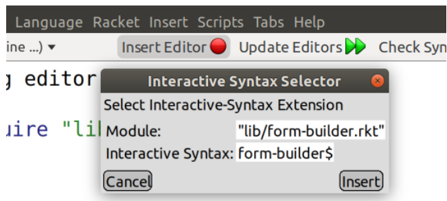
Fig. 11. Inserting an editor inside of DrRacket
