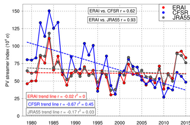
FIG. 12. The 1979–2015 time series of June–November PVSI for ERAI (red line), CFSR (blue line), and JRA-55 (gray line). Trend lines for the 37-yr period are depicted for each dataset (dashed lines). Correlation ( r ) between ERAI and the other two datasets are depicted at the top, and the correlation and r^2 values for each reanalysis trend lines are depicted in the bottom left.
