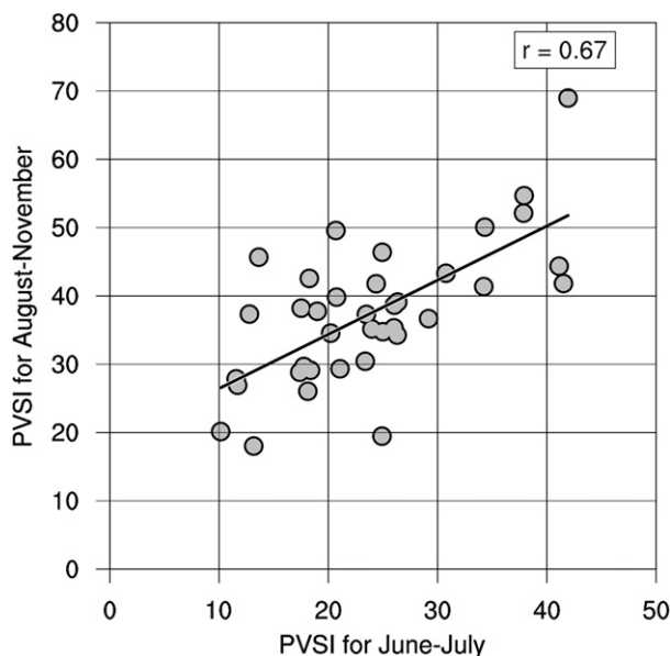
FIG. 10. Scatterplot of the 1979–2015 PVSI early in the TC season (June–July; x axis) compared to total PVSI later in the TC season (August–November; y axis). A linear best-fit (black line) and correlation (at top right) between early and later PVSI are also depicted. The correlation is statistically significant at the 95% confidence interval using bootstrap resampling with 10 000 resamples (Wilks 2006). Data are from ERAI.
