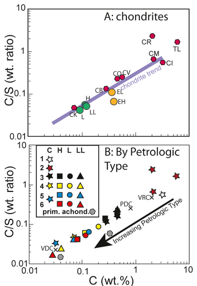
Fig. 1. C and S compositions of chondrite meteorite groups plotted as log C/S versus log C, following Hirschmann (34). (A) Average compositions of different chondrite groups; (B) average compositions of carbonaceous and ordinary chondrites, sorted by petrologic type, plus average compositions of primitive achondrite groups, acapulcoites, and winonaites. Data sources are given in SI Appendix, Table S1. Also shown are three model compositions used in calculations: VRC (volatile-rich chondrite), PDC (partially degassed chondrite), and VDC (volatile-depleted chondrite).
