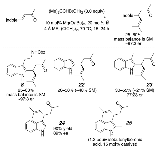
Figure 5. Indole control experiments.
