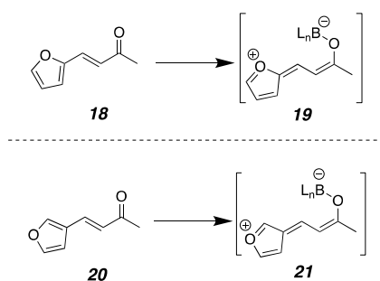
Figure 4. Resonance stabilization of Lewis acid/base interactions.
