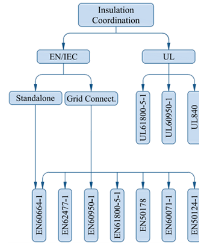
Fig. 4. Insulation coordination process.
