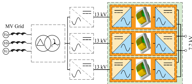
Fig. 8. Converter structure for the case study.
