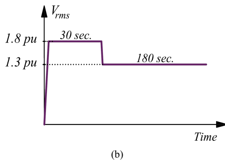
Fig. 3. a) Partial discharge test setup, b) Partial discharge test procedure according to IEEE Std. C57.124 and IEC 60076-11.
