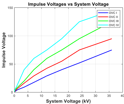
Fig. 5. Impulse voltages according to system voltage for OVC I to OVC IV.
