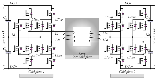
Fig. 10. A single stage of the converter for the case study.
