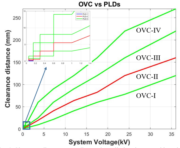
Fig. 6. Clearance distance according to the pollution degree and impulse voltage.
