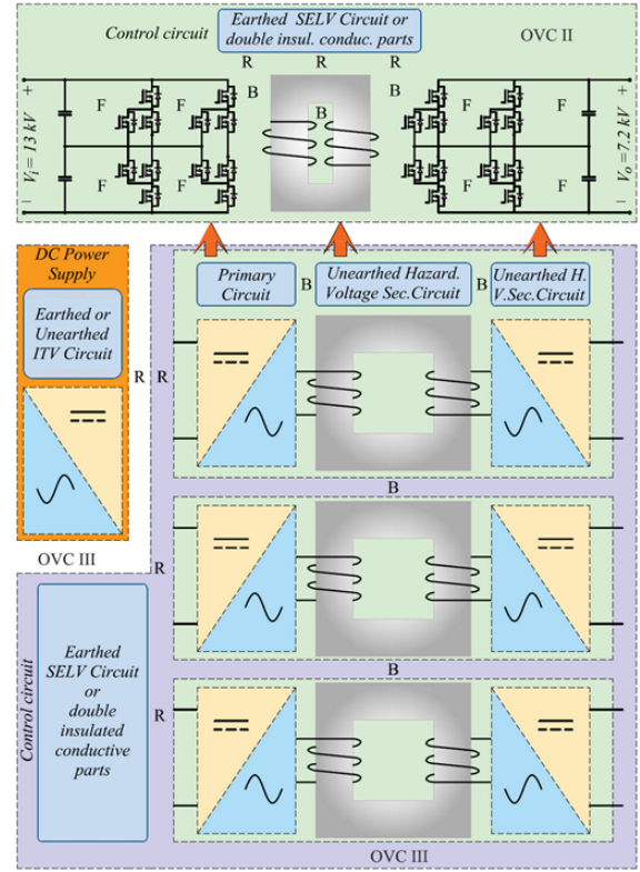
Fig. 9. Required insulation and OCV levels for the case study converter.
