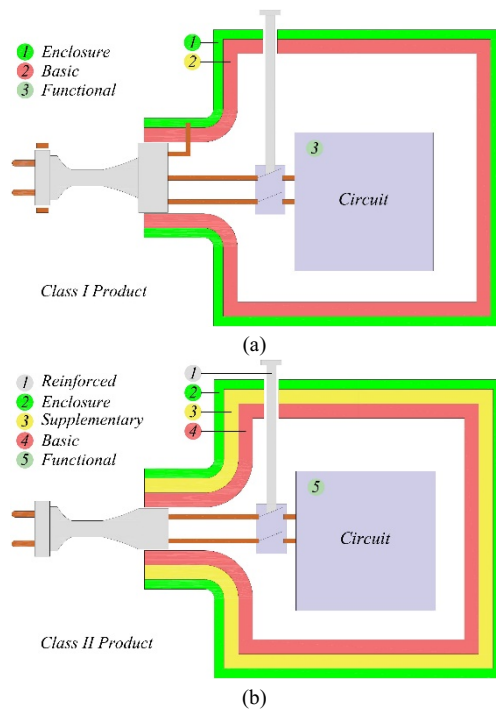
Fig. 2. Use of these insulation types a) In Class-I, b) In Class-II systems.
