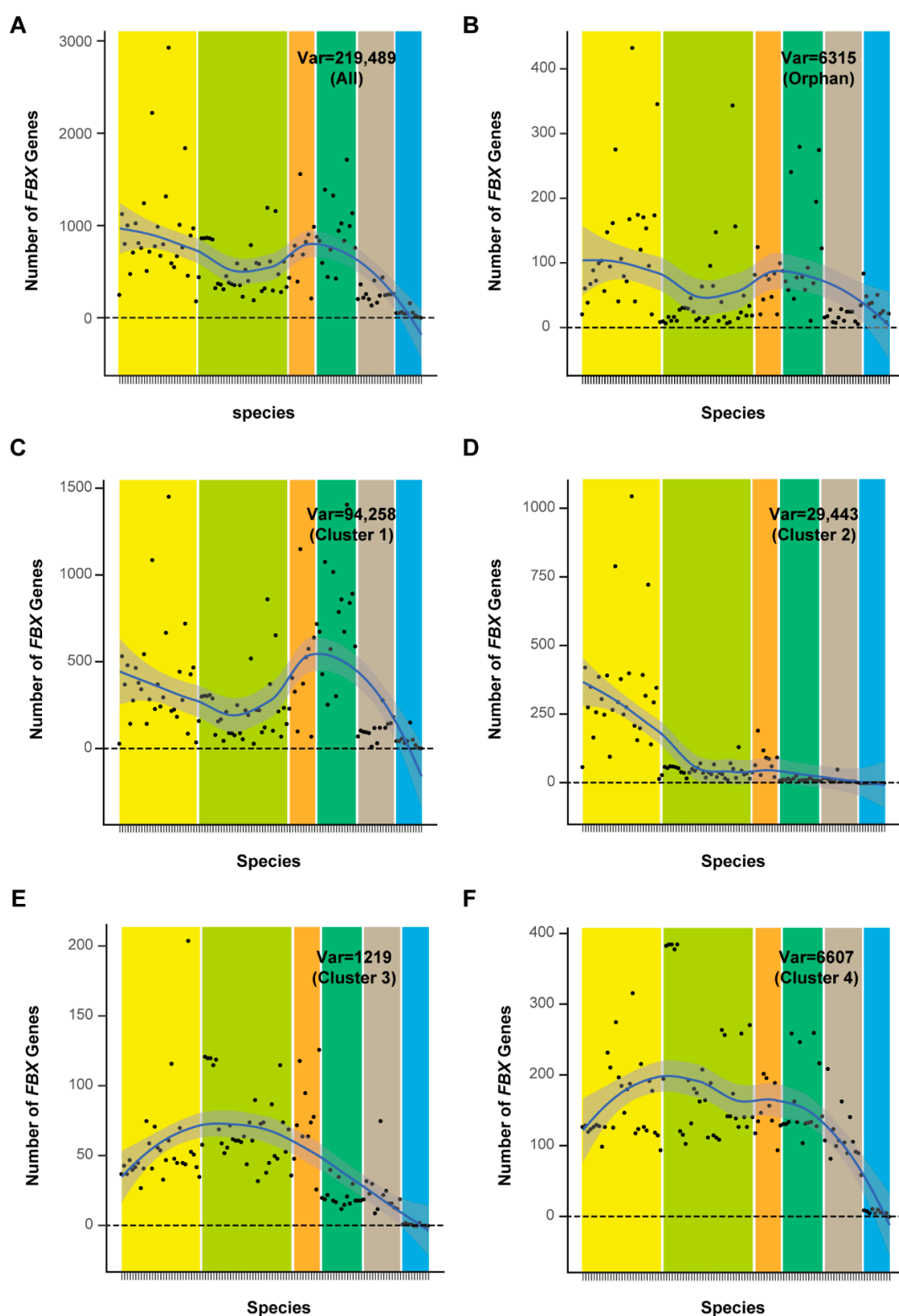
Figure 5. Variation in the number of FBX genes in different groups in 111 plant genomes. The solid blue line and shaded area represent the LOESS (Local Regression) fits \pm 95\% confidence interval in each panel. The value of number variation is also indicated. The yellow, light green, orange, dark green, gray, and cyan bars ordered from left to right in each panel indicate six groups of plants that belong to Brassicales, non-Brassicale rosids, non-rosid dicots, Poaceae, basal embryophytes, and algae, respectively. The vertical lines in the x-axis represent 111 plant genomes that are grouped and listed in an order as in Figure 8A. (A) The complete set of FBX subfamilies. (B) The group of orphan FBX genes. (C) Cluster 1 FBX subfamilies. (D) Cluster 2 FBX subfamilies. (E) Cluster 3 FBX subfamilies. (F) Cluster 4 FBX subfamilies.
