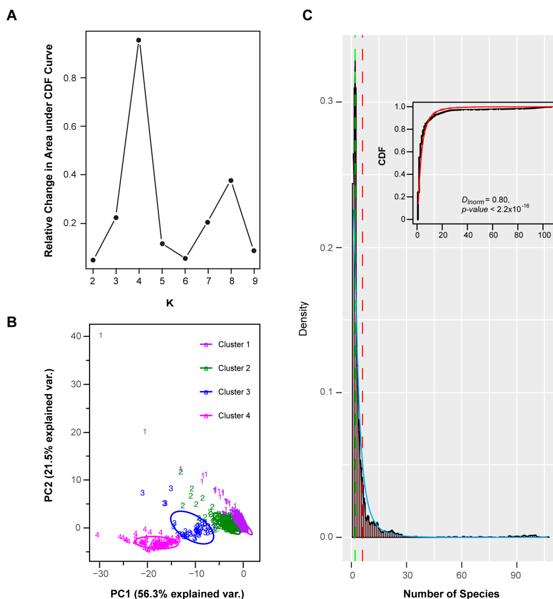
Figure 3. Multi-dimensional features of the FBX subfamilies. (A) A delta area plot analyzed by ConsensusClusterPlus based on the number of species, phylogenetic distance, missing species, and the maximum and mean number of FBX genes per plant of each subfamily demonstrates four optimal k-mean clusters of FBX subfamilies. (B) A bi-dimensional plot showing the first two dimensions of a principal component analysis (PCA) of multi-dimensional features of the FBX subfamilies. PC1 accounts for 56.3% of the variance between individuals and PC2 accounts for 21.5%. Colored data points indicate the four clusters obtained from the analysis in (A) . (C) The distribution of FBX subfamilies is biased toward lineage-specificity more strongly than expected under a random model, suggestive of strong selection. Dashed red and green lines indicate the mean and mode number of species in a subfamily, respectively. Solid black and cyan lines indicate empirical and expected density curves under a log-normal distribution, respectively. The inset shows the curves of the empirical (black dots) and expected (red line) cumulative distribution function (CDF) under a log-normal distribution model. The Kolmogorov–Smirnov test indicates that the empirical and expected CDF curves do not fit.
