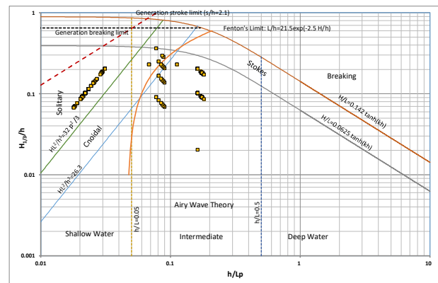
Figure 5 - Wave conditions tested, defined in front of the wave machine. The plot includes the regions of validity for different wave theories.
