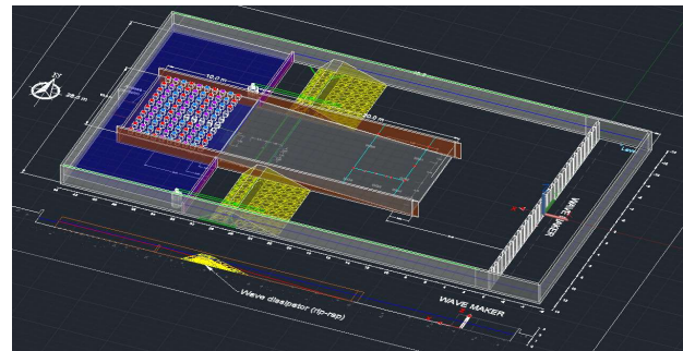
Figure 1 - CAD rendering of the DWB at Oregon State University depicting the foreshore bathymetry and developed barrier island, as well as the recirculation sections to generate steady overland flow.
