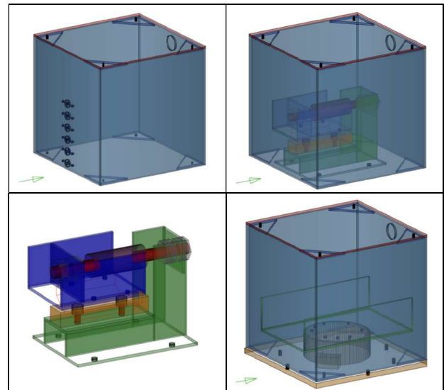
Figure 4 - Design of (a) coastal structure fitted with pressure gauges; (b) coastal structure fitted with in-line axial load cells; (c) the mini-reaction frame to measure axial loads on each of the coastal structures; and (d) coastal structure fitted with a multi-axial load cell.
