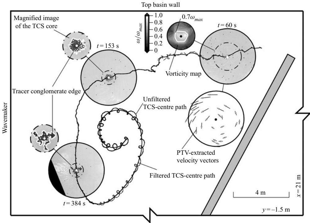
Figure 17. Illustration of the methodology for the extraction of the TCS-centre for one of the experimental trials. In the early stages of TCS development, the density of tracers around the TCS-centre is sufficient to interpolate the velocity field, and the centre is extracted through vorticity maps. In the next stages of TCS development, the TCS-centre is defined as the centre of mass of the tracer conglomerate edge. The extracted vortex path is subsequently filtered to remove the oscillations around the true TCS-centre. All images are plotted to scale except the TCS core images showing the edge detection, which are scaled by a factor of two.
