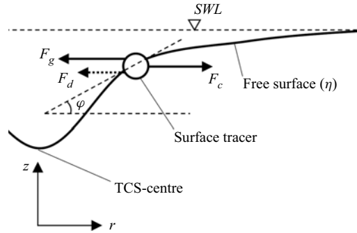
Figure 20. Forces acting on a surface tracer in the radial direction: F_c is the centrifugal force, F_g is the horizontal component of the gravitational force and F_d is the drag force.
