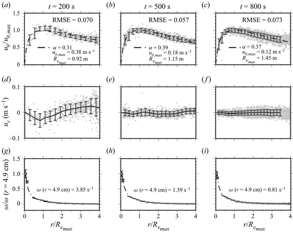
Figure 11. (a–c) Azimuthal velocity ( u_\theta ) profiles normalised with u_{\theta,max} : grey dots correspond to scattered data, error bars to the azimuthal-averaged values and standard deviation, and the dash-dot line to the best-fitting a -profile; root mean square error (RMSE) values correspond to the dimensionless RMSE between the normalised best-fitting a -profile and scattered data for the radial range shown ( r/R_{vmax} \leq 4 ). (d–f) Radial velocity ( u_r ) profiles: grey dots correspond to scattered data, error bars and solid line to the azimuthal-averaged values and standard deviation. (g–i) Azimuthal-averaged vertical vorticity profiles, normalised using the cross-tracer-measured vorticity: the solid line is the azimuthal-averaged vorticity (plotted for r \geq 40 cm), grey circle and square (and corresponding error bars) denote the cross-tracer and square-tracer-measured vorticity, respectively, the grey dots correspond to the scattered vorticity data evaluated on the regular evaluation grid described in § 2.5.1, and the dash-dot line is the theoretical vorticity profile given by (3.14). The abscissa of all subplots is normalised by R_{max} , the radius corresponding to u_{\theta,max} , derived from the best-fitting a -profile.
