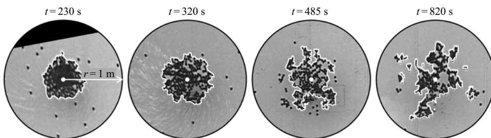
Figure 16. The edge of the tracer conglomerate at the TCS-centre (white polygons) detected through image processing. The rectified images, extracted from a single experimental trial at the times shown in the titles, are centred around the TCS-centre (white circles). At the early stages of TCS development, flow convergence keeps the tracer conglomerate compact and in one piece. As time progresses, the flow becomes weakly divergent and the tracer conglomerate expands and breaks up into smaller fractions.
