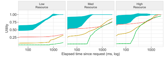
Figure 10: Convergence rate of utility: average utility (y-axis) over time after the user stops on a request.
