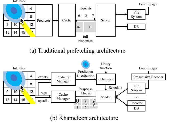
Figure 2: Comparing KHAMELEON to a traditional prefetching architecture for an image exploration DVE application. The interface is a 4 \times 4 grid of image thumbnails. The cursor moved over images 16 and 11 (yellow line) and is now positioned over image 7; the probability of the mouse’s future position is a gaussian distribution illustrated by the blue ellipses (center is the highest probability). The gray boxes are sized according to response sizes. KHAMELEON separates the predictor from the cache, sends probability distributions instead of explicit requests, and uses a scheduler to determine the sequence of small request blocks to send to the client.
