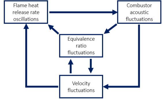
FIGURE 1. Combustion instability feedback loop
