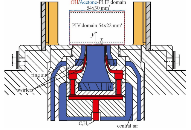
FIGURE 2. Experimental setup with fields of view for three diagnostics.
