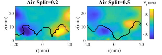
FIGURE 8. Snapshots of the Fourier reconstruction of the radial velocity component at the peak oscillation frequency.
