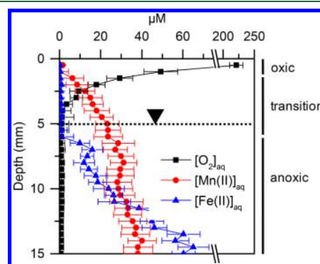
Figure 1. Electrochemistry profiles of dissolved \text{O}_2 , \text{Mn(II)} , and \text{Fe(II)} concentrations across the soil column. Depth is measured relative to the surface of the soil column in the reactor. Profiles represent the average of three replicate reactors, with error bars denoting the standard error of the mean. “Oxic,” “transition,” and “anoxic” zones were sampled for solid phase analysis. The position of the stationary water table is indicated by the dotted line.
