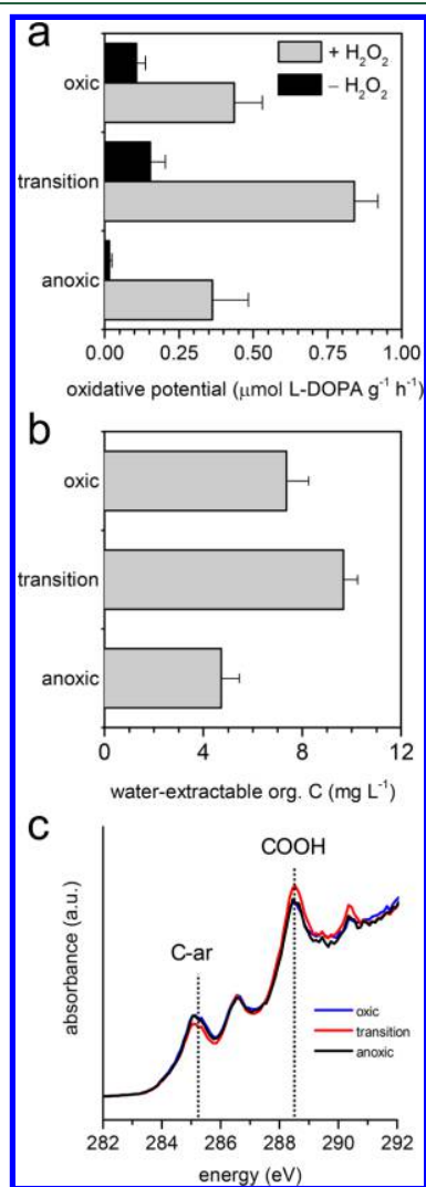
Figure 3. Carbon oxidation across the interface. Changes in (a) oxidative potential for lignin analogue L-3,4-dihydroxyphenylalanine (L-DOPA), (b) the amount of water extractable organic C, and (c) chemical composition of solid-phase C as determined by C K-edge X-ray absorption near-edge spectroscopy (XANES) across the interface.
