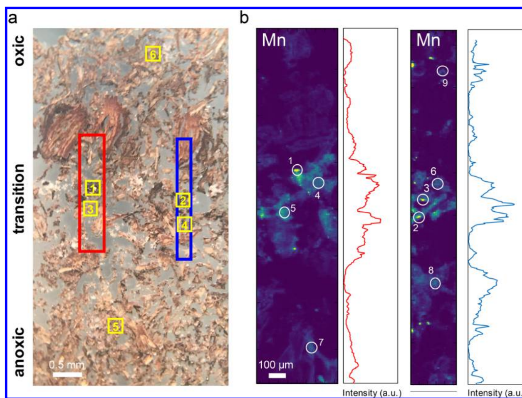
Figure 4. Micron-scale Mn distribution across oxic–anoxic interfaces. (a) Light microscope image of thin section across the oxic–anoxic interface. Note the band of black precipitates along the transition zones. Red and blue boxes denote regions used for XRF mapping of Mn distribution. Yellow squares denote regions used to collect C \mu XANES. Squares 1 and 2 mark locations with black precipitates along the transition, squares 3 and 4 mark locations along the transition without black precipitates, and squares 5 and 6 mark locations in oxic and anoxic zones. (b) Mn maps across the interface for the two regions of interest (red and blue) identified in a. White circles denote locations for which Mn \mu XANES were collected. Locations with high (+Mn, circles 1–3) and low Mn (–Mn, circles 4–6) concentrations were targeted along the transition zone. \mu M XANES were also collected of locations outside of the transition zone (control, circles 7–9).
