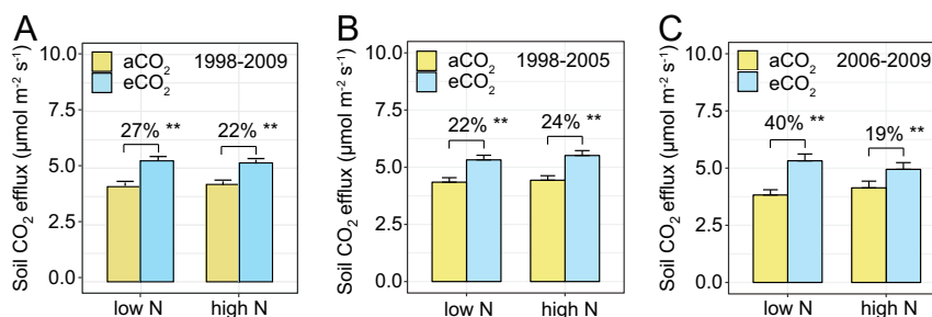
Fig. 1. Observed responses of soil \text{CO}_2 efflux to \text{eCO}_2 at different N supply levels. (A) Soil \text{CO}_2 efflux from 1998 to 2009. (B) Soil \text{CO}_2 efflux from 1998 to 2005 (phase I). (C) Soil \text{CO}_2 efflux from 2006 to 2009 (phase II). Each bar shows the annual mean plus SE of 74 plots. Percent changes of soil \text{CO}_2 efflux in \text{eCO}_2 plots relative to \text{aCO}_2 plots are labeled above the bars. P values of the permutation t test are labeled ** P < 0.01 .
