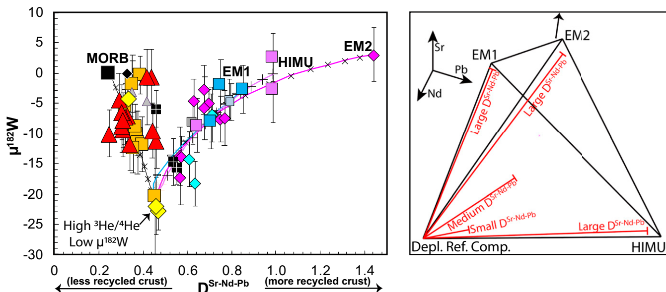
Fig. 5. \mu^{182}\text{W} as a function of D^{\text{Sr-Nd-Pb}} showing that OIB sampling significant recycled crust (represented by extreme EM1, EM2, and HIMU lavas), or MORB, lack \mu^{182}\text{W} anomalies. (Left) Samples with the lowest D^{\text{Sr-Nd-Pb}} (defined in the main text) have the smallest contributions from the EM1, EM2, and HIMU mantle endmembers (and the smallest recycled crust contributions). Samples with the highest D^{\text{Sr-Nd-Pb}} plot closest to EM1, EM2, and HIMU in Sr-Nd-Pb isotopic space (and host the greatest recycled crust contributions). Binary mixing lines are shown between a melt with anomalous \mu^{182}\text{W} and melts of EM1 (blue line), EM2 (pink line), HIMU (purple line), and MORB melts of DM (black mixing line) (see Dataset S6 for model compositions); 10% mixing increments are shown. Symbols are the same as Fig. 3 and data (and 2\sigma errors) are from Dataset S4 (except for OJP data, which are indicated in Fig. 3). (Right) Illustration of calculation of D^{\text{Sr-Nd-Pb}} values and examples of three large D^{\text{Sr-Nd-Pb}} values, one medium D^{\text{Sr-Nd-Pb}} value, and one small D^{\text{Sr-Nd-Pb}} value; all D^{\text{Sr-Nd-Pb}} values are distances in ^{87}\text{Sr}/^{86}\text{Sr} - ^{143}\text{Nd}/^{144}\text{Nd} - ^{206}\text{Pb}/^{204}\text{Pb} isotope space calculated between the depleted reference composition (Depl. Ref. Comp.) and OIB samples.
