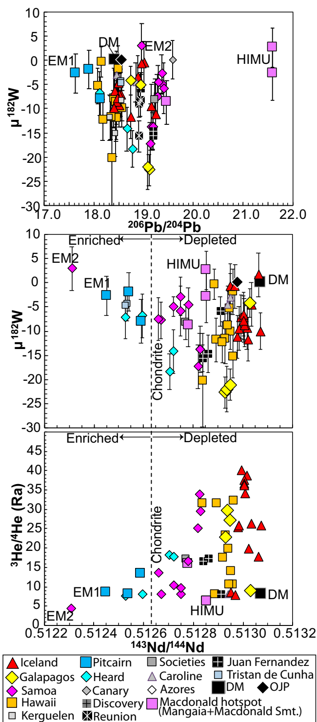
Fig. 3. Relationships between ^3\text{He}/^4\text{He} , \mu^{182}\text{W} , ^{143}\text{Nd}/^{144}\text{Nd} , and ^{206}\text{Pb}/^{204}\text{Pb} in global OIB showing that only geochemically depleted OIB (i.e., high ^{143}\text{Nd}/^{144}\text{Nd} and low ^{206}\text{Pb}/^{204}\text{Pb} ) lacking recycled crust signatures host the highest ^3\text{He}/^4\text{He} and largest-magnitude \mu^{182}\text{W} anomalies. The compilation of He-Sr-Nd-Pb isotopes (from this study and prior studies; Dataset S4 ) for lavas with available \mu^{182}\text{W} shows that only lavas with low ^{206}\text{Pb}/^{204}\text{Pb} (Top) or high ^{143}\text{Nd}/^{144}\text{Nd} (Middle) host the most extreme negative \mu^{182}\text{W} anomalies. Lavas with the most extreme negative \mu^{182}\text{W} anomalies also exhibit high ^3\text{He}/^4\text{He} (Bottom, where only lavas with available \mu^{182}\text{W} data are shown). In contrast, the mantle endmembers EM1, EM2, and HIMU have low ^3\text{He}/^4\text{He} and lack anomalous \mu^{182}\text{W} , as does DM. The chondritic reference ^{143}\text{Nd}/^{144}\text{Nd} is published elsewhere (64). All data and error bars ( 2\sigma ) are provided in Dataset S4 . The ^{143}\text{Nd}/^{144}\text{Nd} and ^{206}\text{Pb}/^{204}\text{Pb} for OJP is an average of
