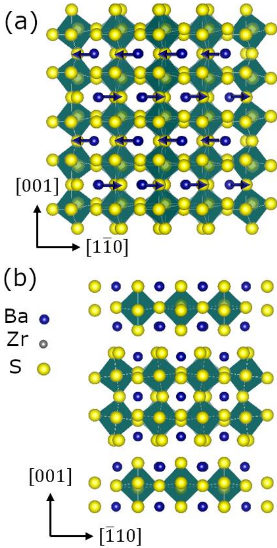
Figure 1: Crystal structures of (a) \text{BaZrS}_3 and (b) \text{Ba}_3\text{Zr}_2\text{S}_7 . The blue, grey and yellow spheres represent Ba, Zr, and S respectively. \text{ZrS}_6 octahedra are shaded in green. The blue arrows indicate the antiferroelectric pattern of \text{Ba}^{2+} cation displacement in \text{BaZrS}_3 .
