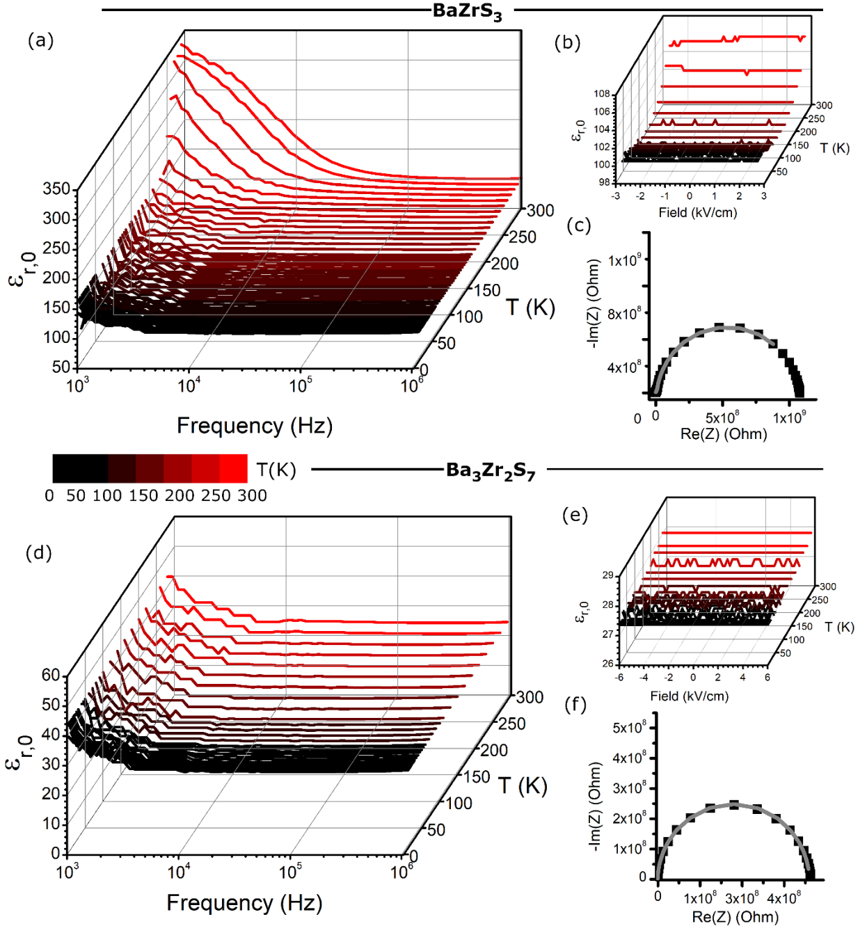
Figure 3: Impedance measurement results for one representative sample each of \text{BaZrS}_3 (a-c) and \text{Ba}_3\text{Zr}_2\text{S}_7 (d-f). (a, d) \epsilon_{r,0} measured for frequency between 1 kHz – 1 MHz and temperature between 2 – 300 K. (b, e) Dependence of \epsilon_{r,0} on an applied electric field. (c, f) Nyquist plot of complex impedance ( Z' - iZ'' ) measured between 0.1 Hz – 1 MHz ambient conditions; points are the data, and line is the fit.
