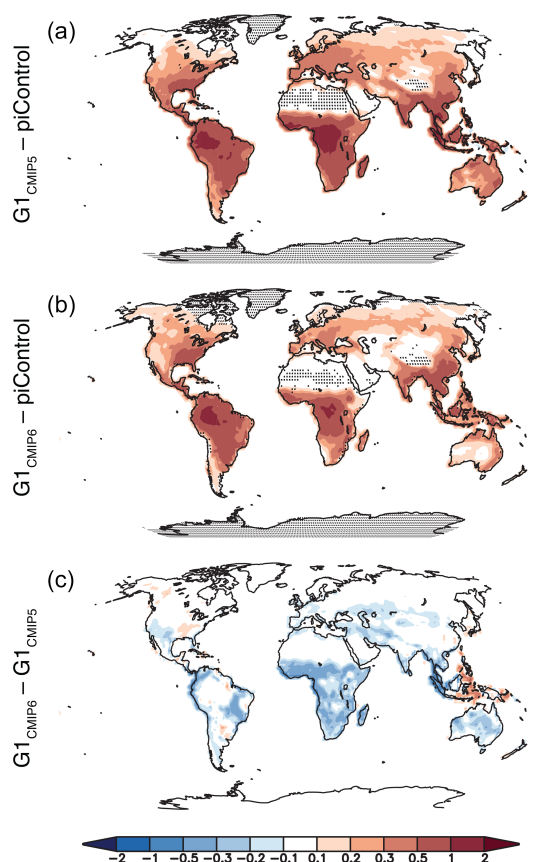
Figure 12. Terrestrial net primary productivity ( \text{kg C m}^{-2} \text{ yr}^{-1} ) for the CMIP5 (a) and CMIP6 (b) ensembles, as well as the ensemble differences (c). All shaded values are ensemble means. Lack of stippling indicates agreement on the sign of the values across at least 75 % of the models.
