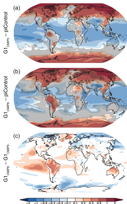
Figure 8. Ensemble average temperature changes (K) for G1 (as compared to the pre-industrial control) for CMIP5 (a) and CMIP6 (b), as well as their difference ( G1_{\text{CMIP6}} minus G1_{\text{CMIP5}} , c). In panels (a) and (b), stippling indicates regions where fewer than 75 % of the models in their respective ensembles agree on the sign of the response.
