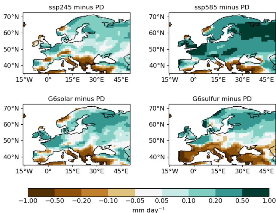
Figure 11. Same as Fig. 10 but for CESM2-WACCM6.
