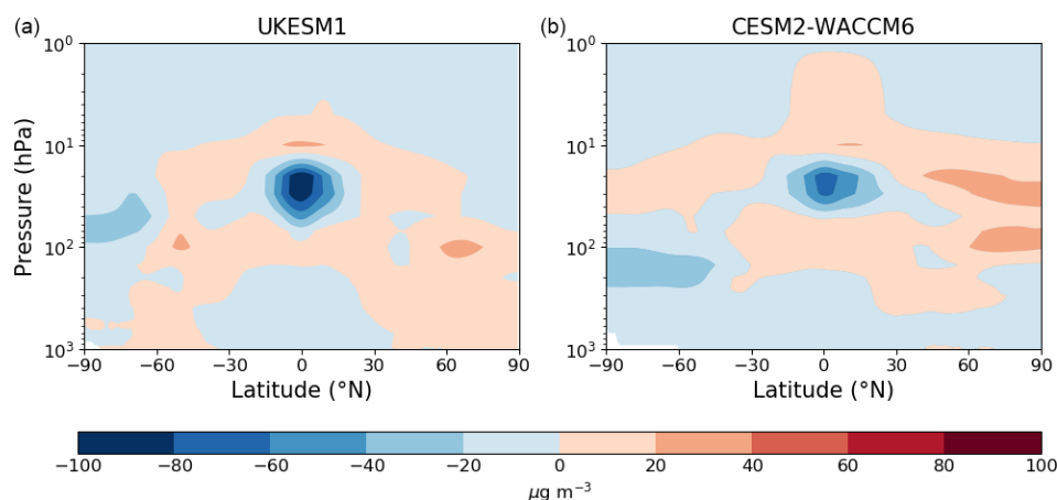
Figure 3. The difference in 2081–2100 annual-mean ozone concentrations (μg m -3 ) diagnosed from {G6sulfur minus G6solar} for UKESM1 (a) and CESM2-WACCM6 (b).
