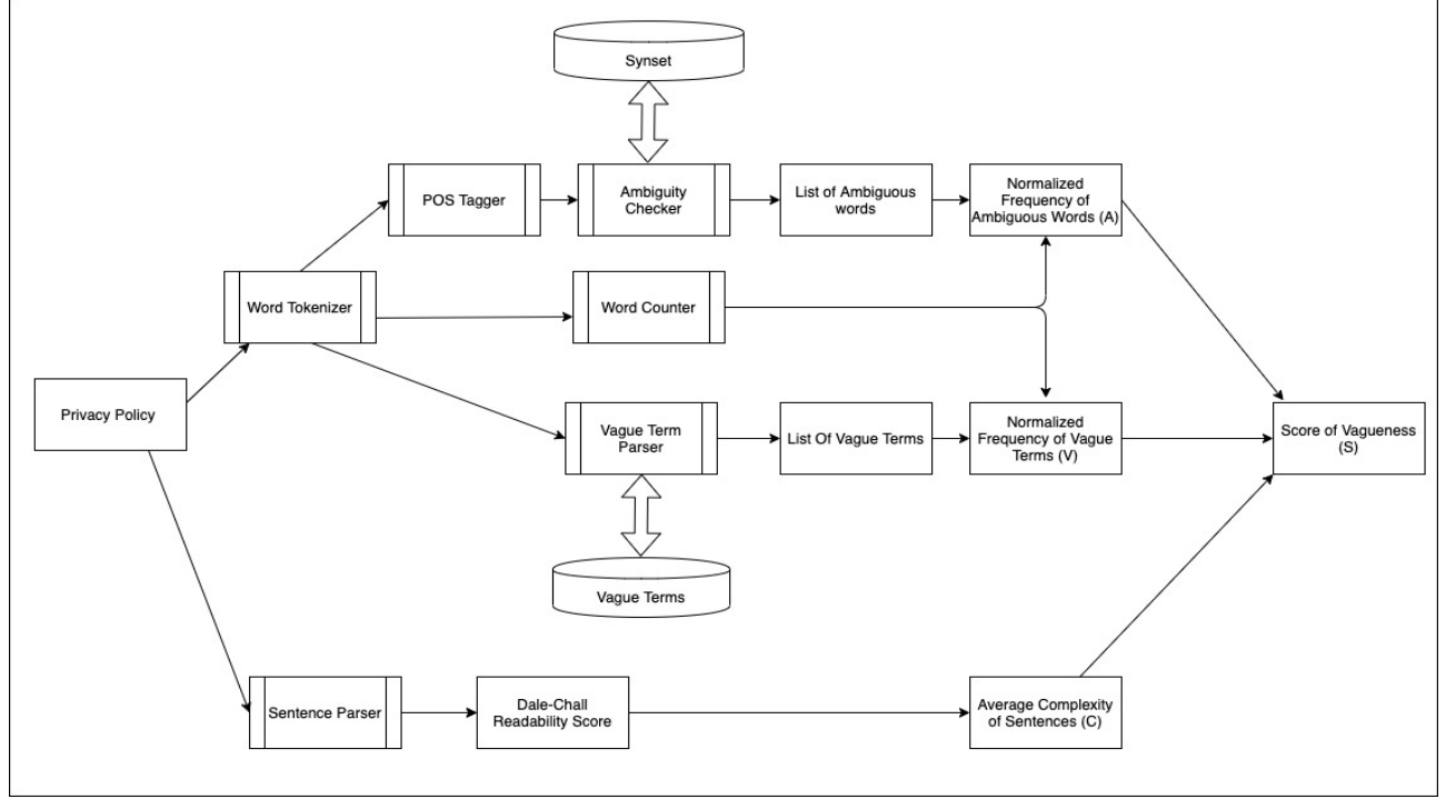
Figure 1: ViCLOUD Architecture
