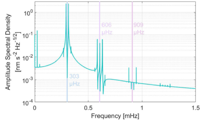
Fig. 3. The theoretical spectrum of a compact HIO undergoing 1-d linear motion near the center of the Earth, on the equatorial plane. The assumed mass of the HIO here is 10^{13} \text{ kg} , and the amplitude of the oscillation is 0.1 r_e . The amplitude spectral density scales approximately as a product of the HIO mass and the the oscillation amplitude. In the spectrum, there are signals centered near the first (around 303 \mu\text{Hz} ) and higher (around 606 \mu\text{Hz} and 909 \mu\text{Hz} ) harmonics due to the non-linearity of the force. Rotation of the Earth (seen as a small lowest-frequency peak) also leads to splitting of the first- and second-harmonic lines. Note that the existence and degree of the splitting is not generic, and can vary depending on the particular orbit. The calculation assumes rigid Earth but goes beyond equation (4) by including transverse acceleration and the nonlinearity of the HIO motion. The nonlinearity leads to the second and higher harmonics of the spectrum, while the transverse acceleration additionally leads to the broadening of the spectral lines.
