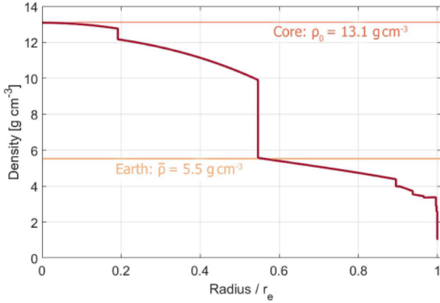
Fig. 1. The density profile of the Earth based on the Preliminary Reference Earth model (PREM) [2]. r_e = 6371 km is the mean radius of the Earth, \bar{\rho} = 5.51 \text{ g cm}^{-3} is the average density of the Earth, and \rho_0 = 13.1 \text{ g cm}^{-3} is the density at the Earth's center.
