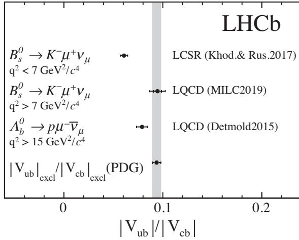
FIG. 2. Measurements of |V_{ub}|/|V_{cb}| in this Letter and in Ref. [7] and ratio inferred from the Particle Data Group (PDG) [26] averages of exclusive |V_{ub}| and |V_{cb}| measurements, where the \Lambda_b^0 \rightarrow p\mu^-\bar{\nu}_\mu result is not included. The form factor calculation used in each case is mentioned [31–33].
