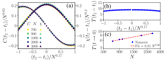
FIG. 3. (a) The correlation and response functions within the stationary state for the type-III quench for different system sizes. t_2 = 20 is chosen to ensure that the stationary state is reached. Scaling collapse is consistent with the exponents \zeta = 1/6 and \alpha = 2/3 . (b) Time-dependent effective temperature T(t) extracted from the two-time correlators for N = 3000 shown in (a). (c) Scaling of T(t) with system size in the limit t \rightarrow 0 . It is consistent with T(t \rightarrow 0) \sim N^{1/3} .
