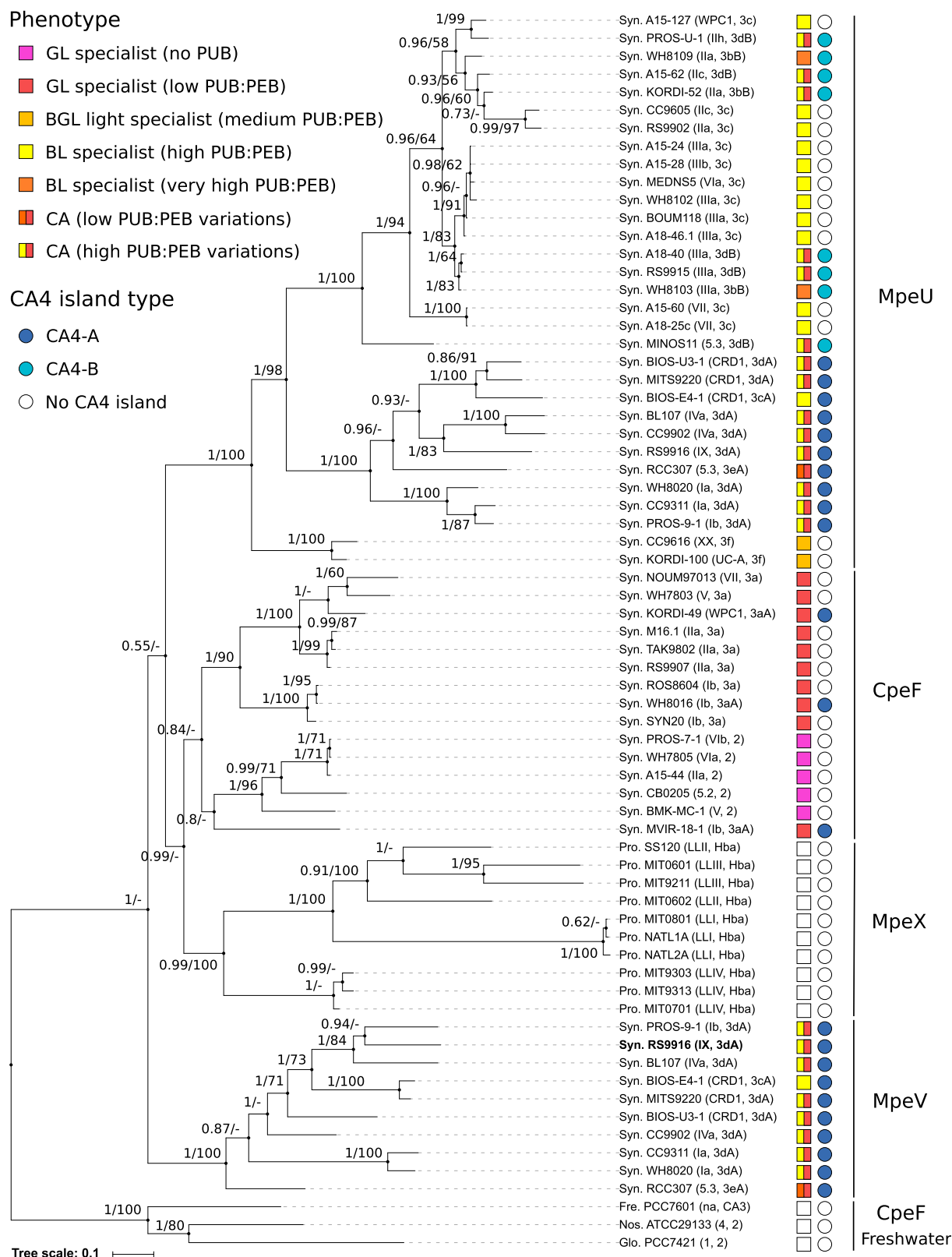
Figure 3. Phylogenetic tree of the MpeV enzyme family. Sequence names include abbreviation of the genus (see below), the strain name, the finest taxonomical level for each strain sensu (67), i.e., subcluster (e.g., 5.2), clade (e.g., VII), or subclade (e.g., IIla), as well as the pigment type sensu (40). The pigment phenotype of each strain is indicated by a colored square and the CA4-island type (A or B) by a blue circle. Strains called “BGL specialists” (light orange square) correspond to strains that are genetically similar to pigment type 3 dB (a.k.a. CA4-B) but that have lost the ability to perform CA4 (i.e., natural CA4 mutants) and are stuck in some intermediate state between the green and blue light phenotype (35). Also worth noting, several strains with a low PUB:PEB ratio have acquired a complete or partial CA4-A island by lateral transfer (pigment type 3aA), but none is CA4-capable (35). Series of two numbers
