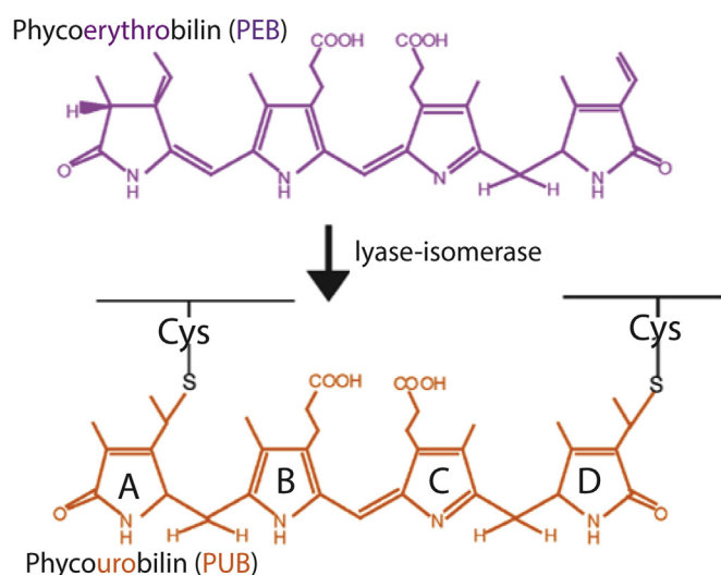
Figure 2. Chemical structures of phycoerythrobilin (PEB) and doubly linked phycourobilin (PUB). Posttranslational pigment attachment is catalyzed by bilin lyases or lyase isomerases with a thioether linkage at the 3 1 carbon of the bilin A ring during single attachment or additionally through the 18 1 carbon of the bilin D ring when doubly attached.
