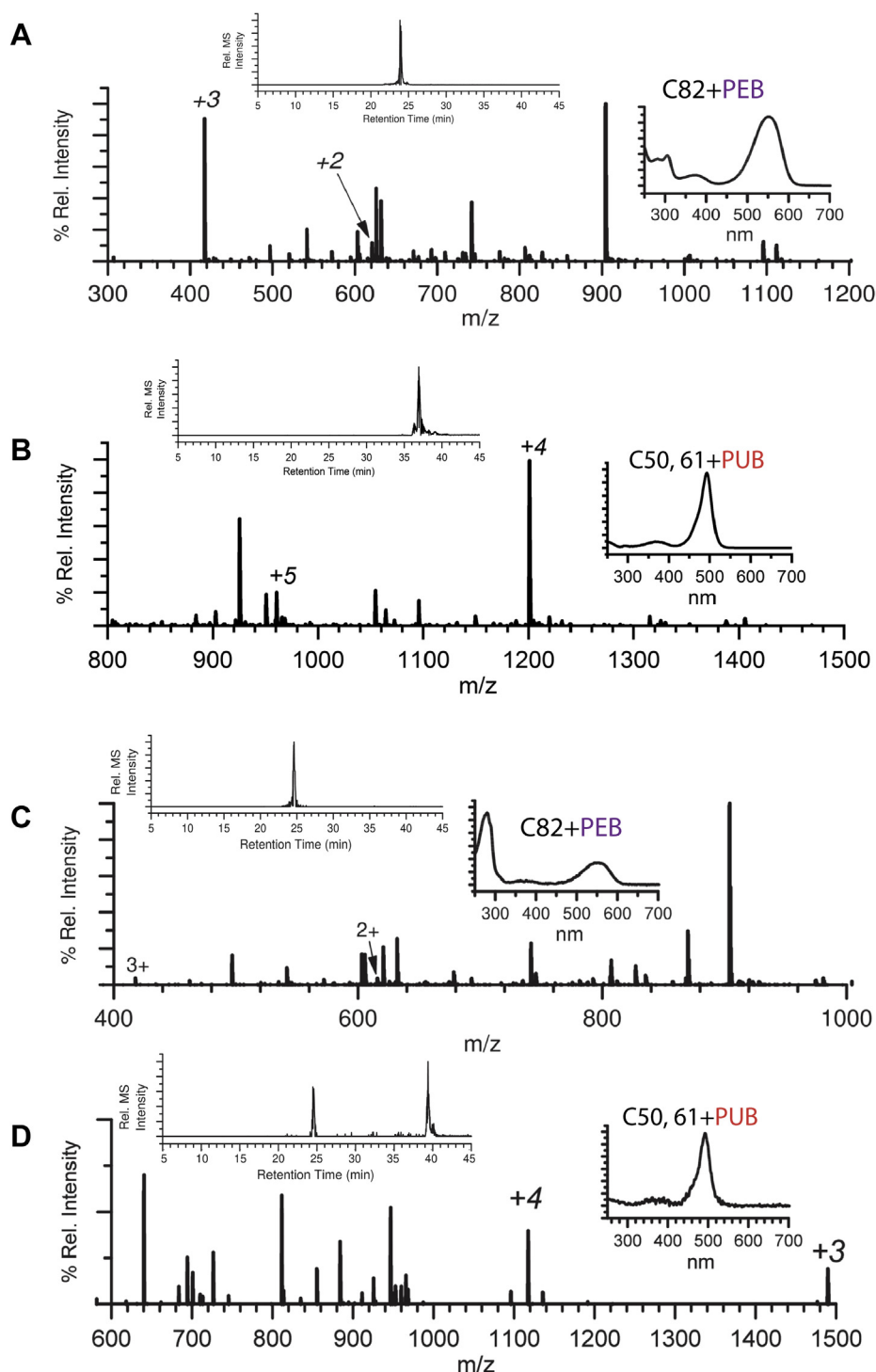
Figure 5. Extracted ion chromatograms and LC-MS spectra for tryptic-digested peptides from RS9916 recombinant \beta -subunits. A, extracted ion chromatogram (EIC, inset left) and LC-MS for the peptide MAAC 82 LR at m/z 417.5 3+ and 625.8 2+ of recombinant RS9916 CpeB C82-PEB (~560 nm). B, EIC (inset left) and LC-MS for peptide LDAVNAITSNASC 50 IVSDAVTGMIC 61 ENTGLIQAGGNCPNRR at m/z 1200.2 4+ and 960.46 5+ of recombinant RS9916 CpeB C50, 61-PUB (~490 nm). C, EIC (inset left) and LC-MS for the peptide KMAAC 82 LRU at m/z 417.5 3+ and 689.5 2+ of recombinant RS9916 MpeB C82-PEB (~560 nm). D, EIC (inset left) and LC-MS for peptide LDAVNAIAGNAAC 50 IVSDAVAGICC 61 ENTGLTAPNGGVYTNR at m/z 1116.8 4+ and 1489.7 3+ of recombinant RS9916 MpeB C50, 61-PUB (~490 nm). Inset right graphs are the UV-visible absorbance spectra for the peaks present in the EIC (inset left). The type of bilin is indicated per panel. All samples expressed in the presence of CpeS, MpeV, CpeZ, and bilin synthesis genes. These results are representative of two independent biological replicates.
