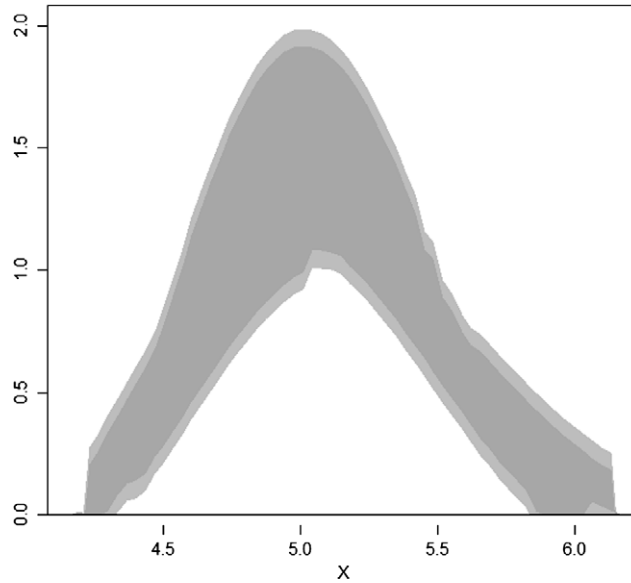
FIGURE 1. 95% confidence band \mathcal{C}_n(0.05) of the density function f_X of the ex post values X of the mineral right in the logarithm of US dollars per acre. The dark gray shade represents the band based on the stochastic part, and the light gray shade represents the uniform bias bound \eta_q .
