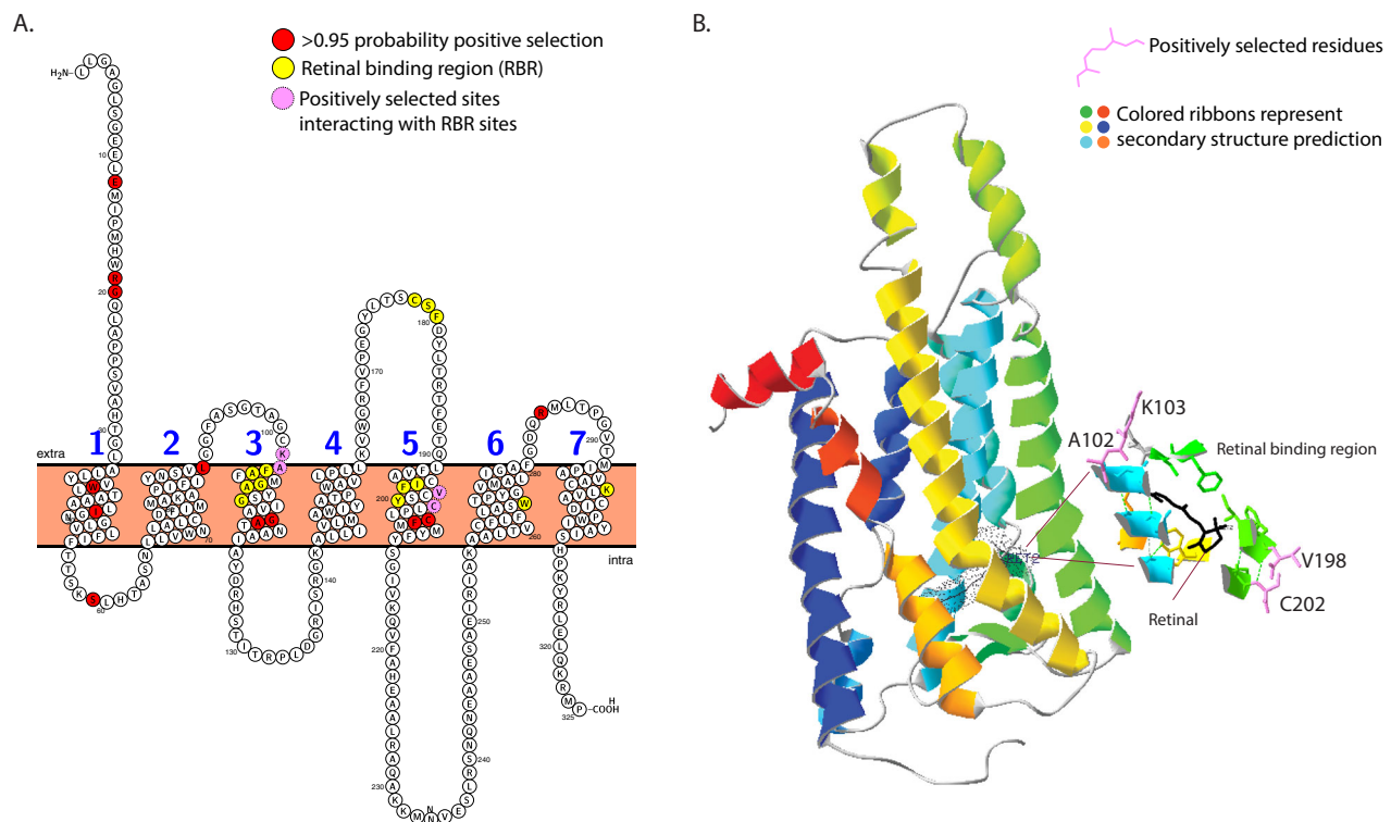
Fig. 3 Opsin structural prediction with retinal binding sites, sites with higher dN/dS (positively selection) and putative tuning sites, the subset that interacts with both. A UV-opsin PHOBIUS transmembrane prediction. Opsins sites with higher dN/dS rates and amino acids close to ( \leq 4 Å) retinal, which form the retinal binding region (RBR) have been marked. B UV-opsin model made using squid rhodopsin as the template. Retinal is marked, secondary structure prediction of alpha helices are shown in different colors and the expanded view shows the positively selected sites that can interact ( \leq 2 Å) with the retinal binding sites. Protein models used to get these metrics can be found at ref. 38 . Sites under positive selection are highlighted in red, sites in the retinal binding region in yellow and positively selected sites that are capable of interacting with the retinal binding sites in pink, identifying likely candidates for opsin tuning ( A ). Other positively selected are located within the transmembrane region and could be indirectly involved in opsin tuning ( B ).
