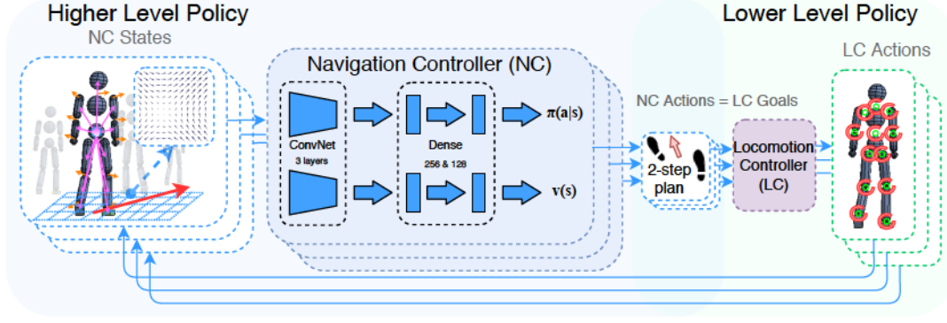
Figure 2: From left to right: the Multi-Agent Navigation Controller (NC) state includes the relative goal position and distance, an egocentric velocity field of the relative velocity of obstacles and other agents, and the agent link positions and linear velocities; for each agent this state is input to a multi-layer Convolutional Neural Network (CNN), including two dense hidden layers, and outputs actions—the value function uses a similar network. These high-level actions, in the form of two-step plans, are given to the Locomotion Controller (LC) as a g , which produces the angle-axis targets for each joint.
