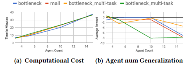
Figure 11: The performance of MAHRL from two quantitative perspectives, (a) the computational performance with respect to agent count and (b) the generalization performance with respect to average reward value. The yellow bottleneck_multi-task curve is a policy learned over multiple environments. The green multi-task curve is a single environment policy tested over multiple environments.
