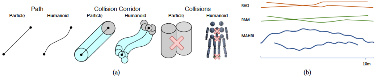
Figure 4: The proposed method is the first of its kind, fundamentally combining physical character control and crowd simulation. Because of this, primary methodologies in comparative crowds analysis have shortcomings which makes methods not representative as outline in (a). First the humanoid’s centre of mass trajectory forms a piecewise parabolic curve unlike particle models where the same path is a straight line. Similarly, the underlying humanoid representation is composed of several capsule and sphere colliders, making the collision corridor and collision detection of the humanoid more complicated, whereas particle models can only detect collision within their particle bounds—typically a single circle or capsule. (b) compares the final trajectories of RVO[48], PAM [20], and MAHRL in a typical oncoming collision task between two agents.
