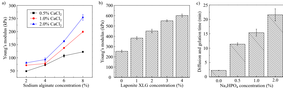
FIGURE 5: Investigations of Young's modulus and diffusion/gelation time of the alginate-based inks. (a) Young's modulus as a function of alginate and \text{CaCl}_2 concentrations. (b) Young's modulus as a function of Laponite XLG concentration. (c) Diffusion and gelation time as a function of \text{Na}_2\text{HPO}_4 concentration. (Error bars: means \pm standard deviation ( SD ) with n = 3 samples per group.)
