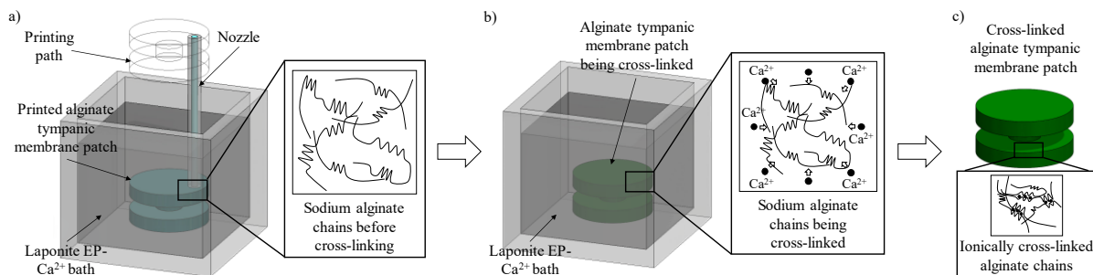
FIGURE 3: Fabrication mechanism of alginate-based tympanic membrane patches. Alginate-based tympanic membrane patch (a) printing and (b) ionic cross-linking in the Laponite EP- \text{CaCl}_2 bath. (c) Schematic of completely cross-linked alginate-based tympanic membrane patch.
