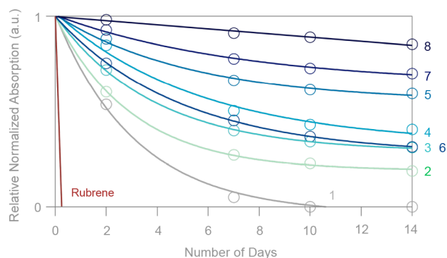
Figure 4. Stability of tetracene materials over a 2 week period when stored in a well-lit (conventional fluorescent tube lighting) aerobic environment. Plot shows \lambda_{\max} intensity relative to intensity on day 0.
