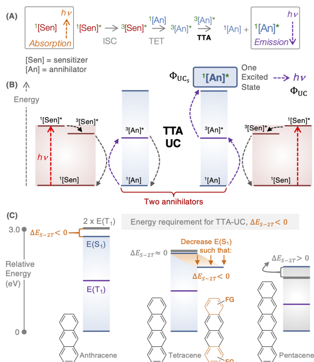
Figure 1. Energetic landscape of TTA-UC. (A) Net process of TTA-UC, where the notation m[\text{Molecule}]^* represents the multiplicity, m , of the systems involved and the asterisk corresponds to excited states (no asterisk corresponds to a ground state molecule). (B) Jablonski diagram of the process of TTA-UC: the sensitizer 1[\text{Sen}] is excited with low-energy light; the singlet exciton 1[\text{Sen}]^* undergoes intersystem crossing (ISC) to a triplet exciton 3[\text{Sen}]^* , which then undergoes triplet energy transfer (TET) to the annihilator 3[\text{An}]^* ; and, finally, the interaction between two 3[\text{An}]^* yield one annihilator in the ground state 1[\text{An}] and other in the singlet state 1[\text{An}]^* by triplet–triplet annihilation. (C) Relative energies 26 E(S_1) and E(T_1) of three molecules that undergo TTA, singlet fission (SF), and competing pathways. The strategy to access the TTA channel in tetracene derivatives by lowering E(S_1) with functional groups (FG), while maintaining E(T_1) fixed, is the focus of this paper.
