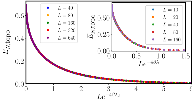
FIG. 3. Scaling collapse of topological negativity in 2D toric code as \lambda_B \rightarrow \infty [Eq. (3)]. L is the size of the bipartition boundary, \beta is the inverse temperature, and \lambda_A is the coefficient for star operators A_s . Inset: scaling collapse of topological negativity in 2D toric code at \lambda = \lambda_A = \lambda_B using a classical Monte Carlo method combined with a transfer matrix method.
