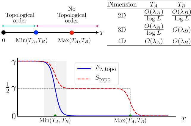
FIG. 1. Upper panel: phase diagram of toric code models. The critical temperatures T_A and T_B corresponding to the proliferation of two types of excitations depend on the spatial dimension. Lower panel: comparison between topological entanglement negativity E_{N,\text{topo}} and topological von Neumann entropy S_{\text{topo}} in toric code models of size L . As L \rightarrow \infty , E_{N,\text{topo}} = 0 for T > \text{Min}(T_A, T_B) , consistent with the absence of topological order while S_{\text{topo}} remains nonzero in the regime \text{Min}(T_A, T_B) < T < \text{Max}(T_A, T_B) . When \text{Min}(T_A, T_B) \neq 0 as L \rightarrow \infty , the behavior of E_{N,\text{topo}} shown close to the critical point (=the shaded region) is just a schematic and we do not probe that region.
