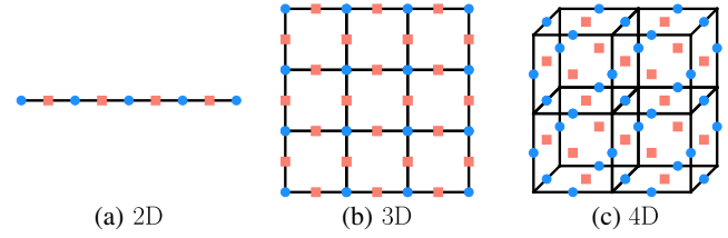
FIG. 2. The boundary operators in toric code for various spatial dimensions. Blue circles and red squares label A_i and B_j operators, respectively. (a) One-dimensional bipartition boundary in 2D toric code, where A_i live on sites, and B_j live on links. (b) Two-dimensional bipartition boundary in 3D toric code, where A_i live on sites, and B_j live on links. (c) Three-dimensional bipartition boundary in 4D toric code, where A_i live on links, and B_j live on faces.
