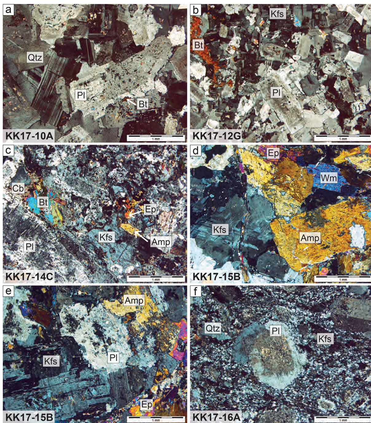
Fig. 3. Representative photomicrographs of the studied samples: (a) anhedronal plagioclase from granite sample KK17-10A, (b) quartz monzonite sample KK17-12G comprising mainly plagioclase and alkali feldspar, (c) altered syenite sample KK17-14C - note mafic minerals: amphibole, biotite and epidote, (d) monzodiorite sample KK17-15B consisting mainly of feldspar, plagioclase and amphibole, (e) plagioclase partly replaced by fine grain opaque minerals, the sample KK17-15B, (f) quartz, plagioclase and feldspar rich granite sample KK17-16A, plagioclase is commonly affected by sericitization. Abbreviations of mineral: Pl - plagioclase, Kfs - K-feldspar, Qtz - quartz, Bt - biotite, Wm- white mica, Ep - epidote, Amp - amphibole and Cb - carbonate.
